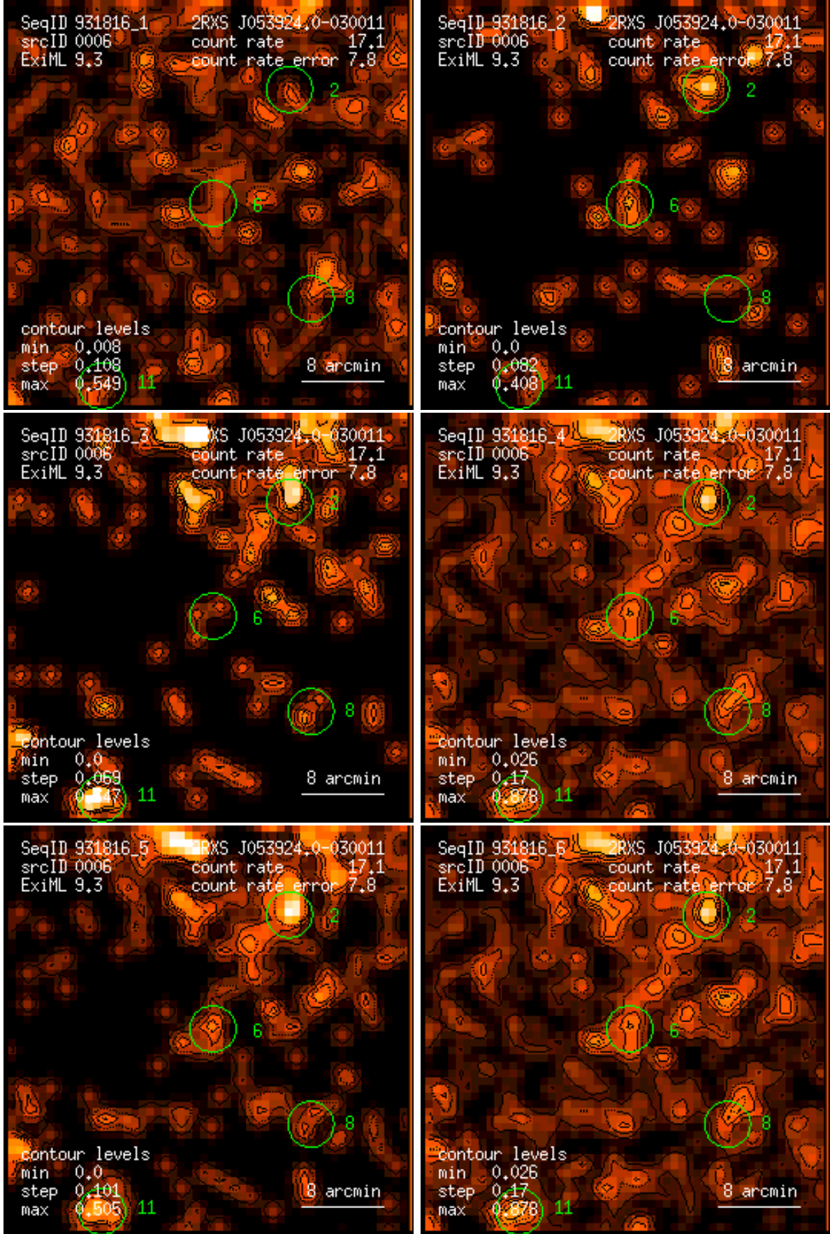
Figure 6: RASS 931816: detection 0006: band rate images, Gaussian filter: (1) PSPC channels 11 – 41, (2) 52 – 90, (3) 91 – 201, (4) 11 – 235, (5) 52 – 201, (6) 11 – 201. Broad band rates in counts/ks. Band rate contour levels in counts/ks/arcmin 2 .
