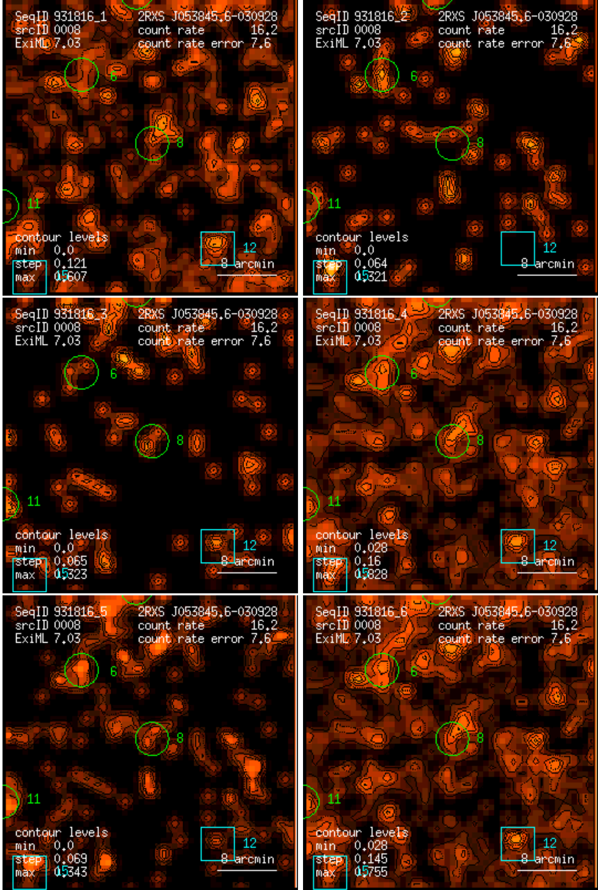
Figure 8: RASS 931816: detection 0008: band rate images, Gaussian filter: (1) PSPC channels 11 – 41, (2) 52 – 90, (3) 91 – 201, (4) 11 – 235, (5) 52 – 201, (6) 11 – 201. Broad band rates in counts/ks. Band rate contour levels in counts/ks/arcmin 2 .
