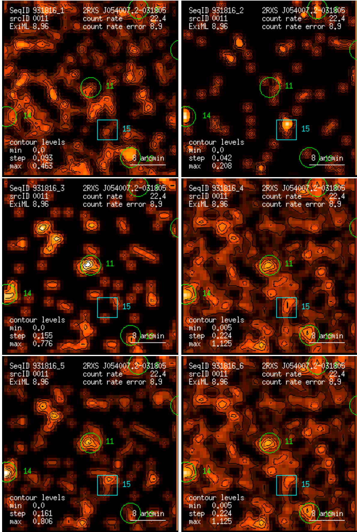
Figure 11: RASS 931816: detection 0011: band rate images, Gaussian filter: (1) PSPC channels 11 – 41, (2) 52 – 90, (3) 91 – 201, (4) 11 – 235, (5) 52 – 201, (6) 11 – 201. Broad band rates in counts/ks. Band rate contour levels in counts/ks/arcmin 2 .
