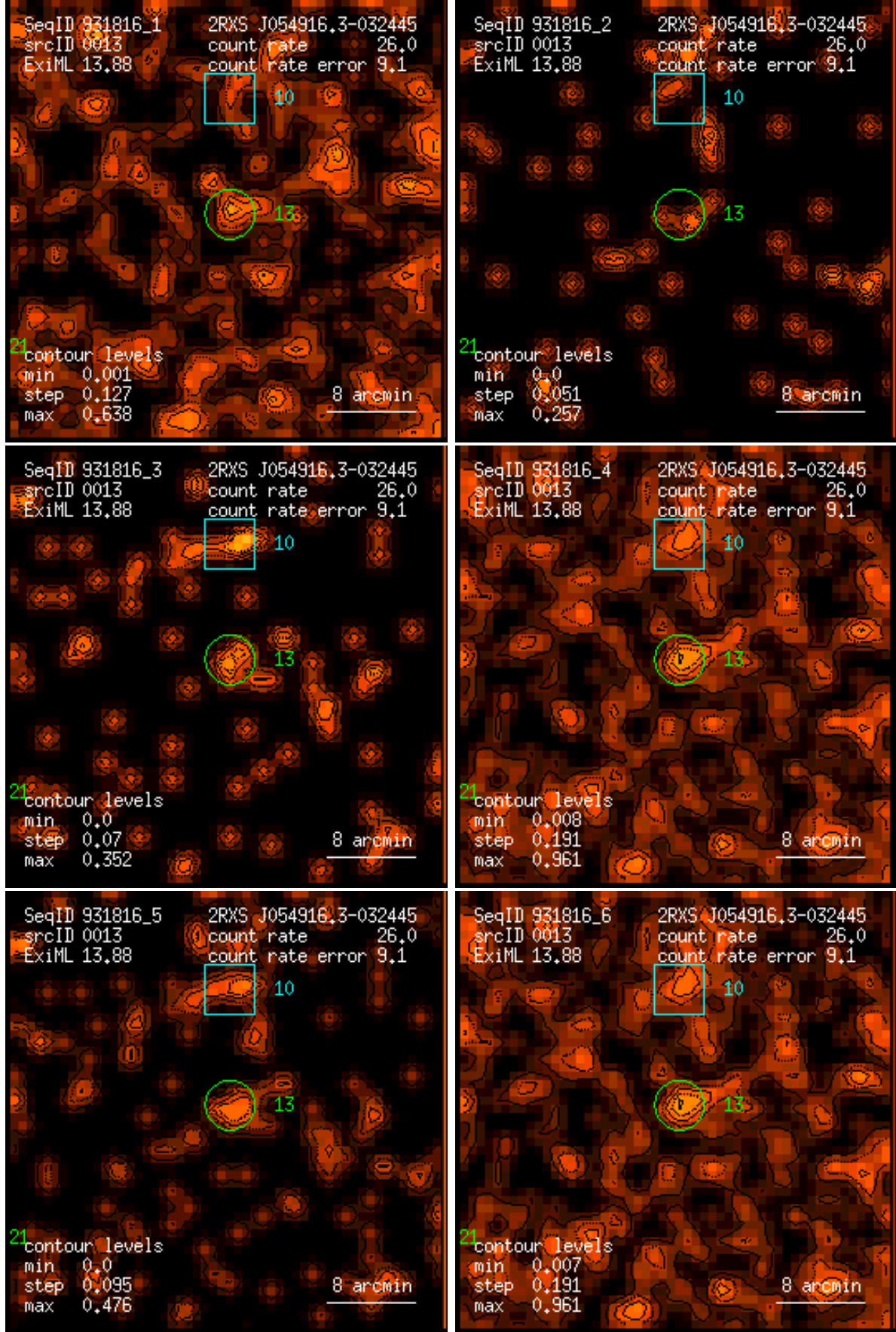
Figure 13: RASS 931816: detection 0013: band rate images, Gaussian filter: (1) PSPC channels 11 – 41, (2) 52 – 90, (3) 91 – 201, (4) 11 – 235, (5) 52 – 201, (6) 11 – 201. Broad band rates in counts/ks. Band rate contour levels in counts/ks/arcmin 2 .
