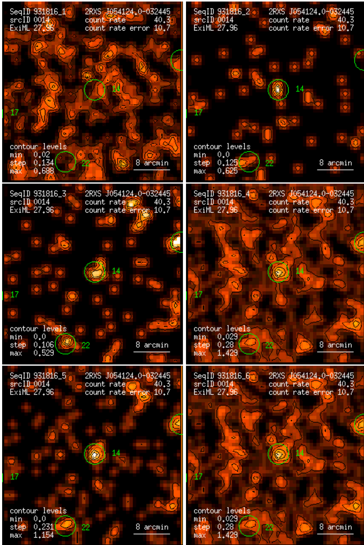
Figure 14: RASS 931816: detection 0014: band rate images, Gaussian filter: (1) PSPC channels 11 – 41, (2) 52 – 90, (3) 91 – 201, (4) 11 – 235, (5) 52 – 201, (6) 11 – 201. Broad band rates in counts/ks. Band rate contour levels in counts/ks/arcmin 2 .
