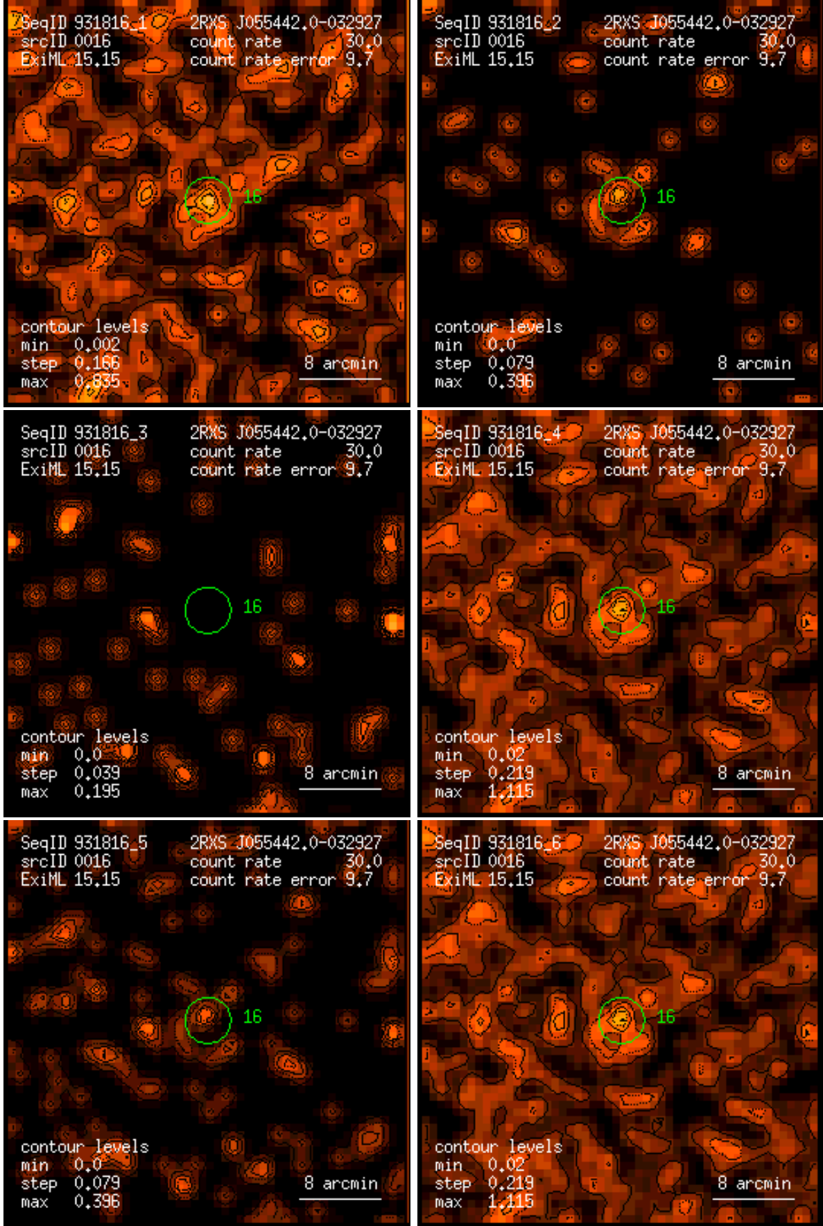
Figure 16: RASS 931816: detection 0016: band rate images, Gaussian filter: (1) PSPC channels 11 – 41, (2) 52 – 90, (3) 91 – 201, (4) 11 – 235, (5) 52 – 201, (6) 11 – 201. Broad band rates in counts/ks. Band rate contour levels in counts/ks/arcmin 2 .
