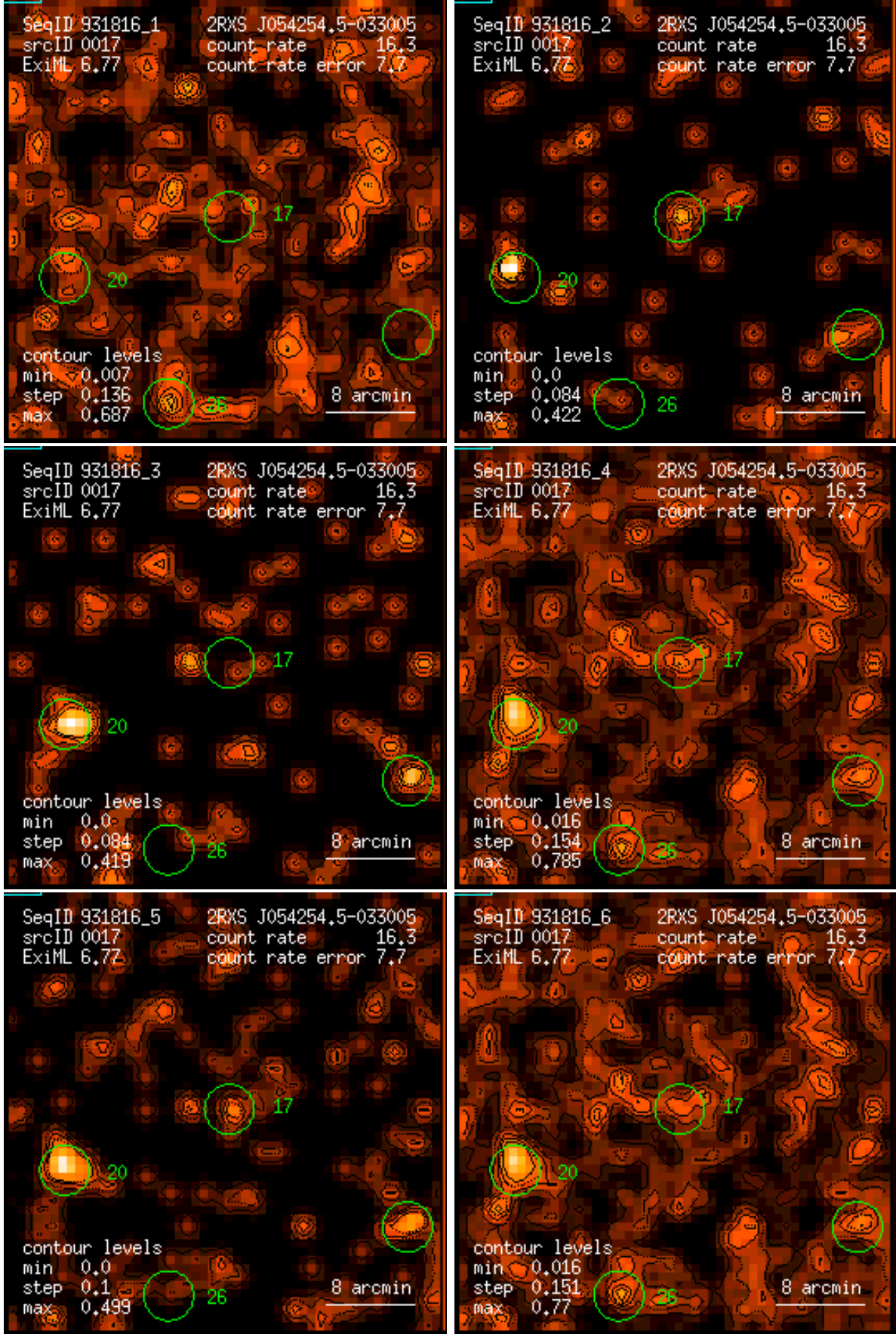
Figure 17: RASS 931816: detection 0017: band rate images, Gaussian filter: (1) PSPC channels 11 – 41, (2) 52 – 90, (3) 91 – 201, (4) 11 – 235, (5) 52 – 201, (6) 11 – 201. Broad band rates in counts/ks. Band rate contour levels in counts/ks/arcmin 2 .
