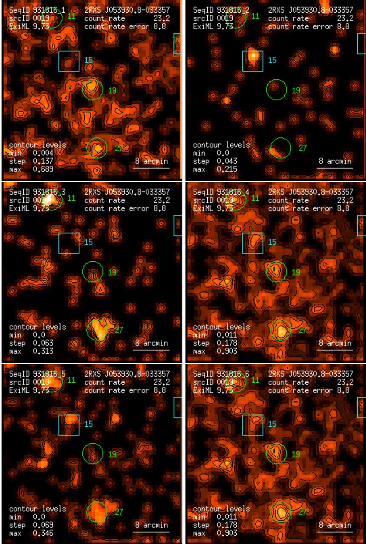
Figure 19: RASS 931816: detection 0019: band rate images, Gaussian filter: (1) PSPC channels 11 – 41, (2) 52 – 90, (3) 91 – 201, (4) 11 – 235, (5) 52 – 201, (6) 11 – 201. Broad band rates in counts/ks. Band rate contour levels in counts/ks/arcmin 2 .
