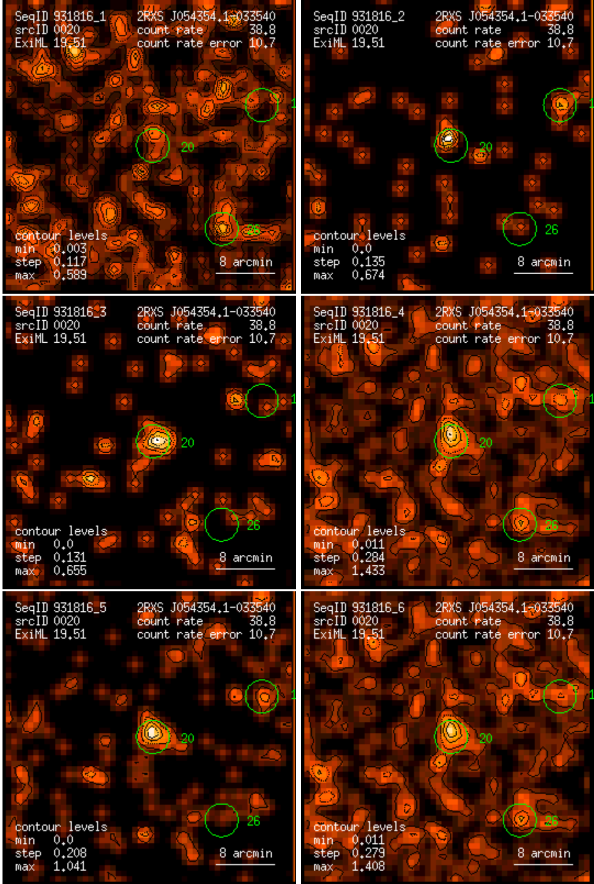
Figure 20: RASS 931816: detection 0020: band rate images, Gaussian filter: (1) PSPC channels 11 – 41, (2) 52 – 90, (3) 91 – 201, (4) 11 – 235, (5) 52 – 201, (6) 11 – 201. Broad band rates in counts/ks. Band rate contour levels in counts/ks/arcmin 2 .
