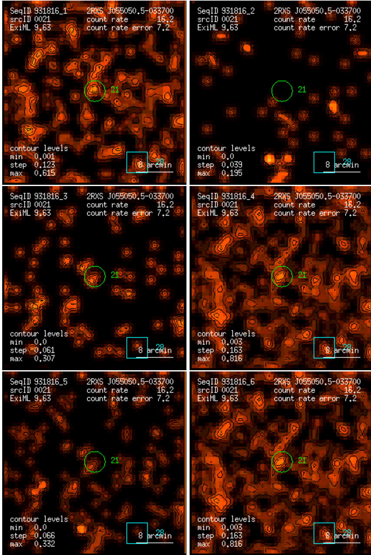
Figure 21: RASS 931816: detection 0021: band rate images, Gaussian filter: (1) PSPC channels 11 – 41, (2) 52 – 90, (3) 91 – 201, (4) 11 – 235, (5) 52 – 201, (6) 11 – 201. Broad band rates in counts/ks. Band rate contour levels in counts/ks/arcmin 2 .
