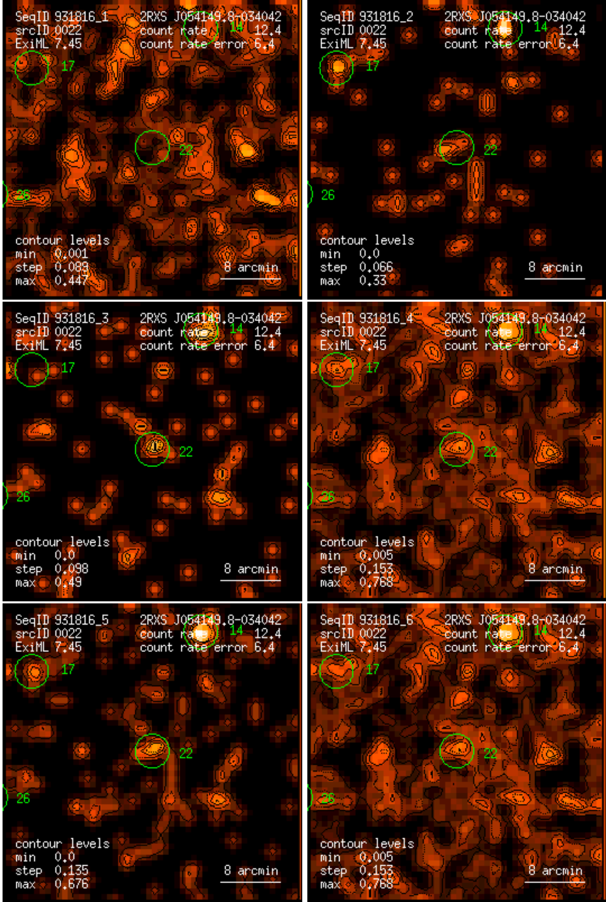
Figure 22: RASS 931816: detection 0022: band rate images, Gaussian filter: (1) PSPC channels 11 – 41, (2) 52 – 90, (3) 91 – 201, (4) 11 – 235, (5) 52 – 201, (6) 11 – 201. Broad band rates in counts/ks. Band rate contour levels in counts/ks/arcmin 2 .
