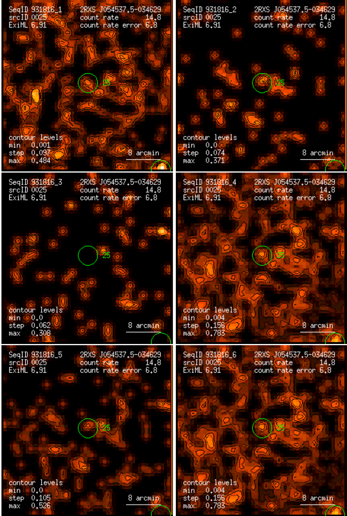
Figure 25: RASS 931816: detection 0025: band rate images, Gaussian filter: (1) PSPC channels 11 – 41, (2) 52 – 90, (3) 91 – 201, (4) 11 – 235, (5) 52 – 201, (6) 11 – 201. Broad band rates in counts/ks. Band rate contour levels in counts/ks/arcmin 2 .
