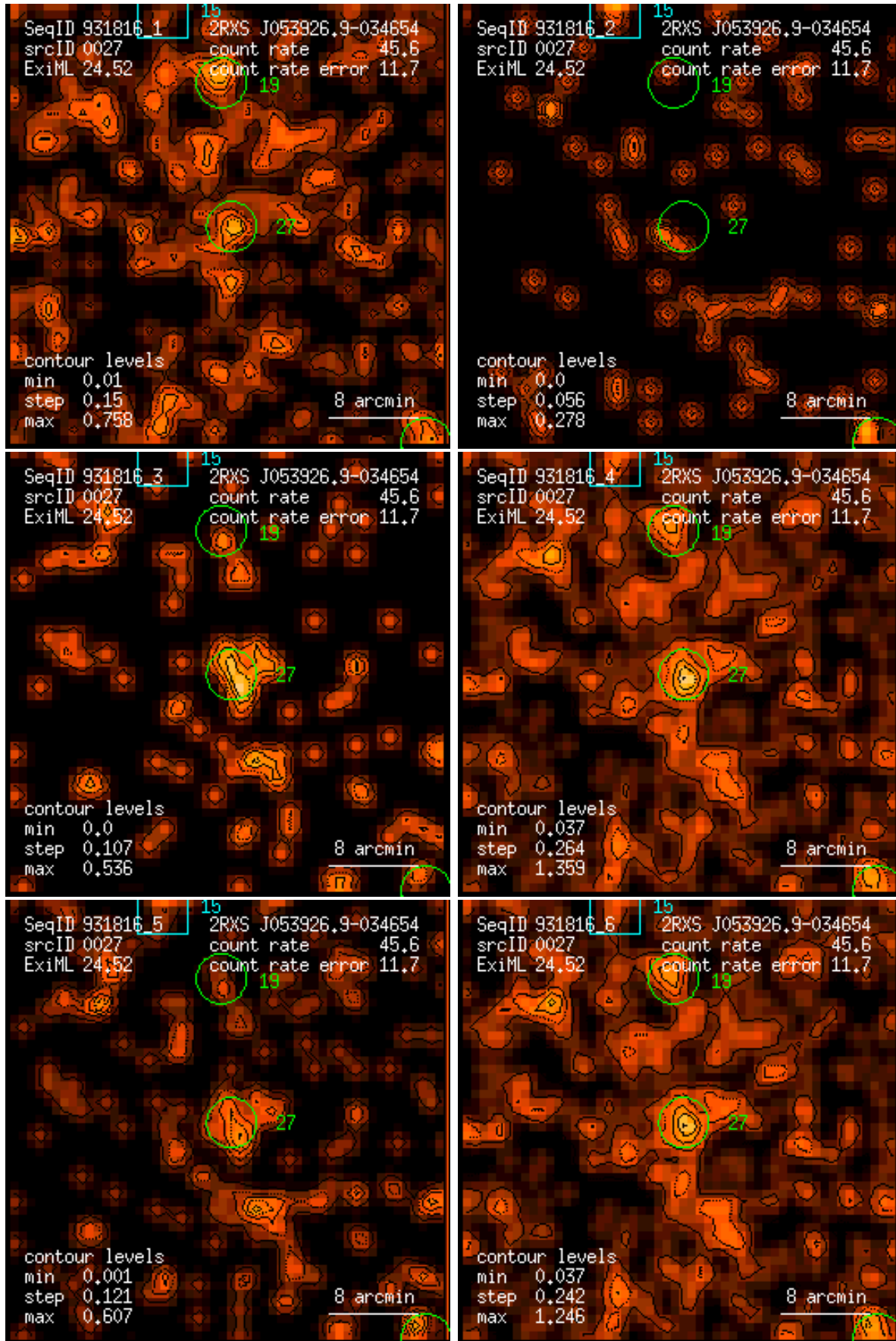
Figure 27: RASS 931816: detection 0027: band rate images, Gaussian filter: (1) PSPC channels 11 – 41, (2) 52 – 90, (3) 91 – 201, (4) 11 – 235, (5) 52 – 201, (6) 11 – 201. Broad band rates in counts/ks. Band rate contour levels in counts/ks/arcmin 2 .
