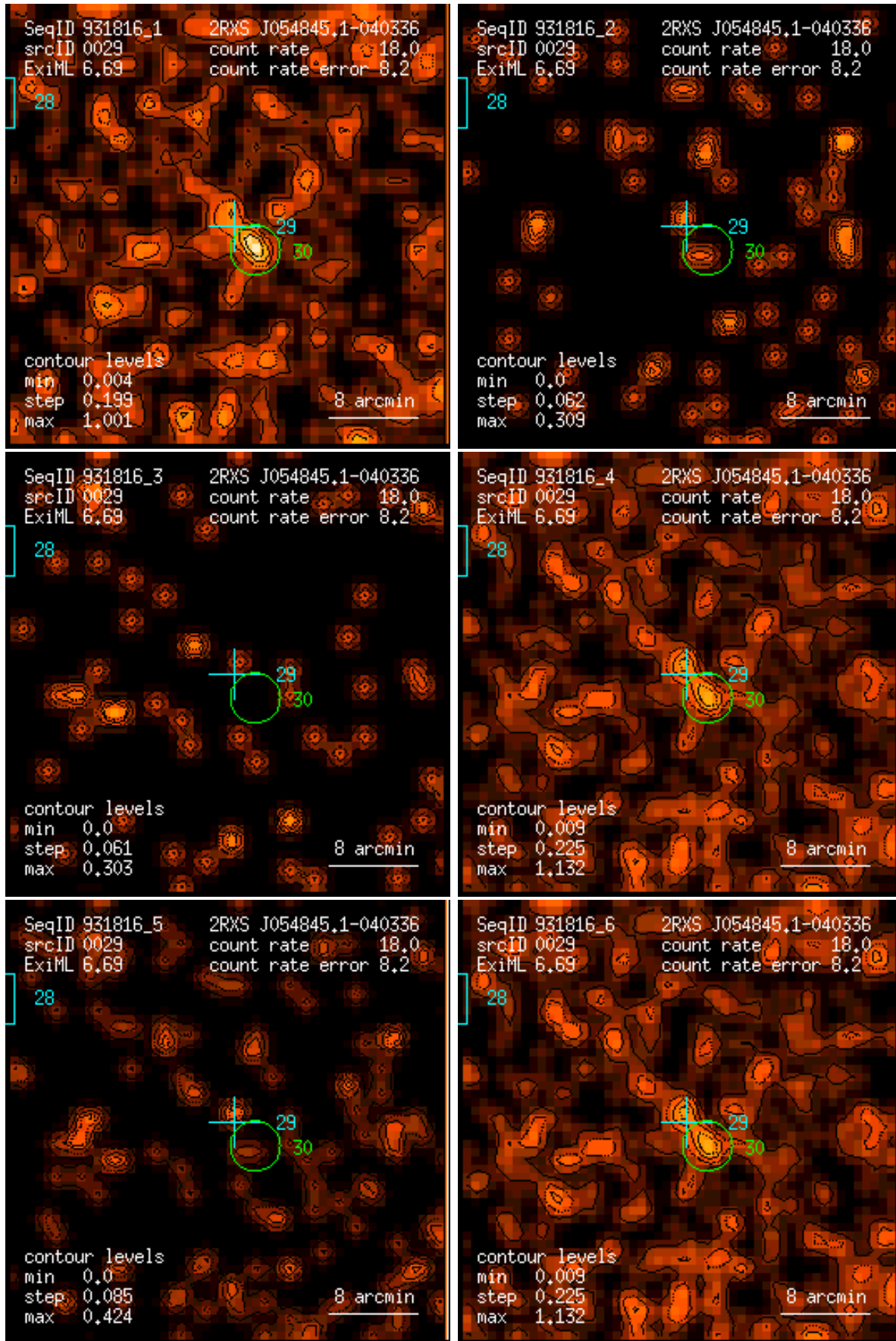
Figure 29: RASS 931816: detection 0029: band rate images, Gaussian filter: (1) PSPC channels 11 – 41, (2) 52 – 90, (3) 91 – 201, (4) 11 – 235, (5) 52 – 201, (6) 11 – 201. Broad band rates in counts/ks. Band rate contour levels in counts/ks/arcmin 2 .
