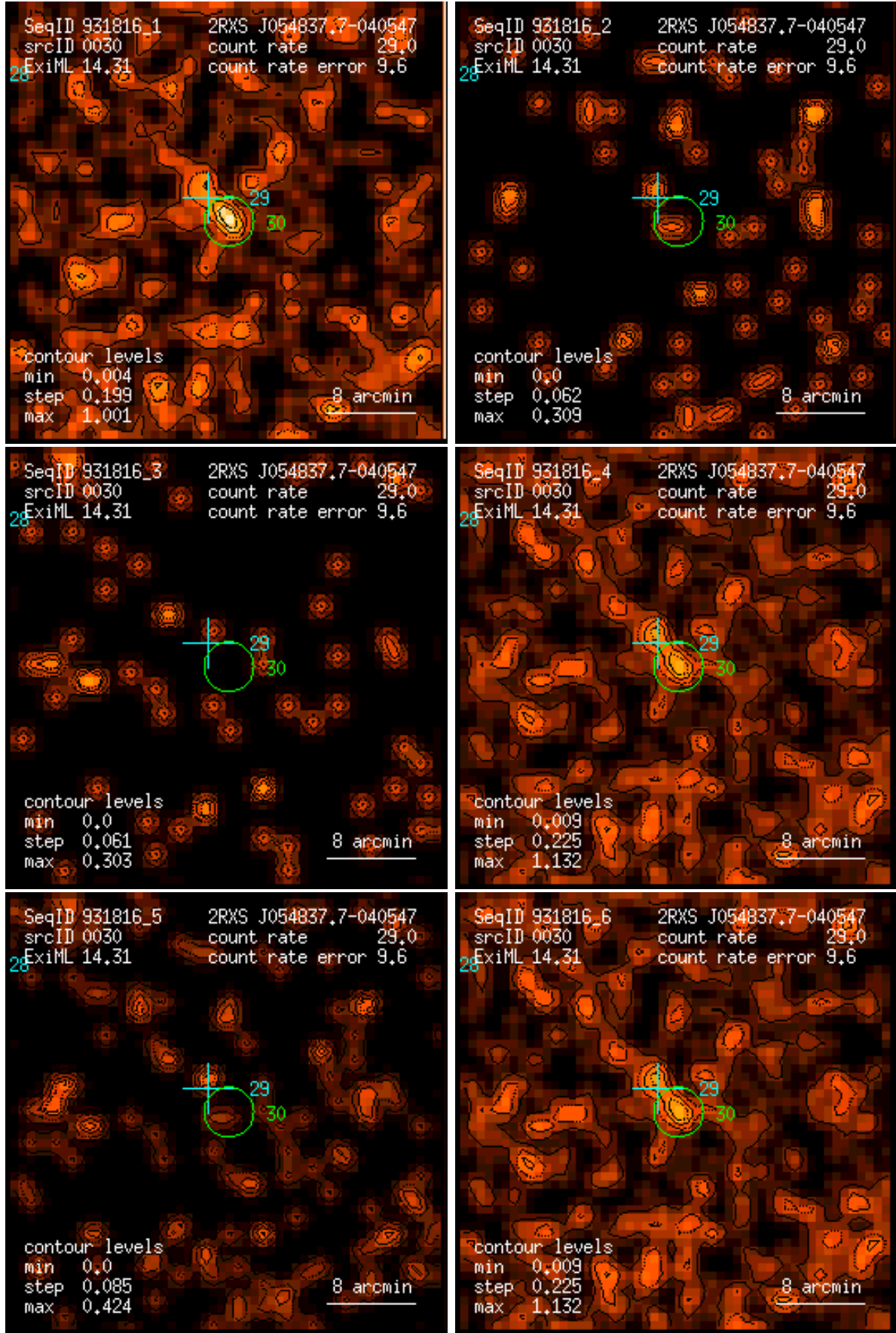
Figure 30: RASS 931816: detection 0030: band rate images, Gaussian filter: (1) PSPC channels 11 – 41, (2) 52 – 90, (3) 91 – 201, (4) 11 – 235, (5) 52 – 201, (6) 11 – 201. Broad band rates in counts/ks. Band rate contour levels in counts/ks/arcmin 2 .
