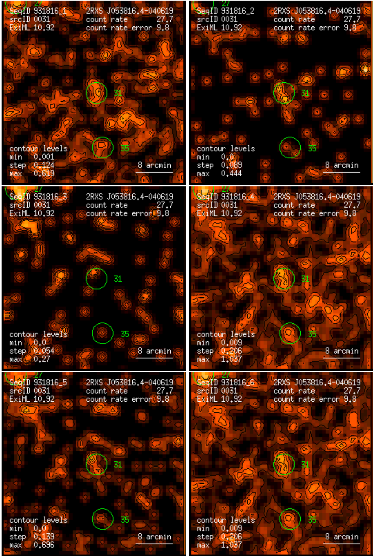
Figure 31: RASS 931816: detection 0031: band rate images, Gaussian filter: (1) PSPC channels 11 – 41, (2) 52 – 90, (3) 91 – 201, (4) 11 – 235, (5) 52 – 201, (6) 11 – 201. Broad band rates in counts/ks. Band rate contour levels in counts/ks/arcmin 2 .
