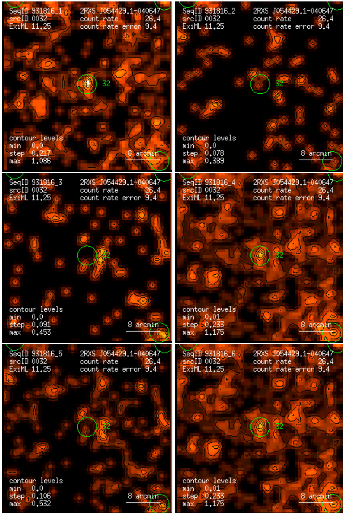
Figure 32: RASS 931816: detection 0032: band rate images, Gaussian filter: (1) PSPC channels 11 – 41, (2) 52 – 90, (3) 91 – 201, (4) 11 – 235, (5) 52 – 201, (6) 11 – 201. Broad band rates in counts/ks. Band rate contour levels in counts/ks/arcmin 2 .
