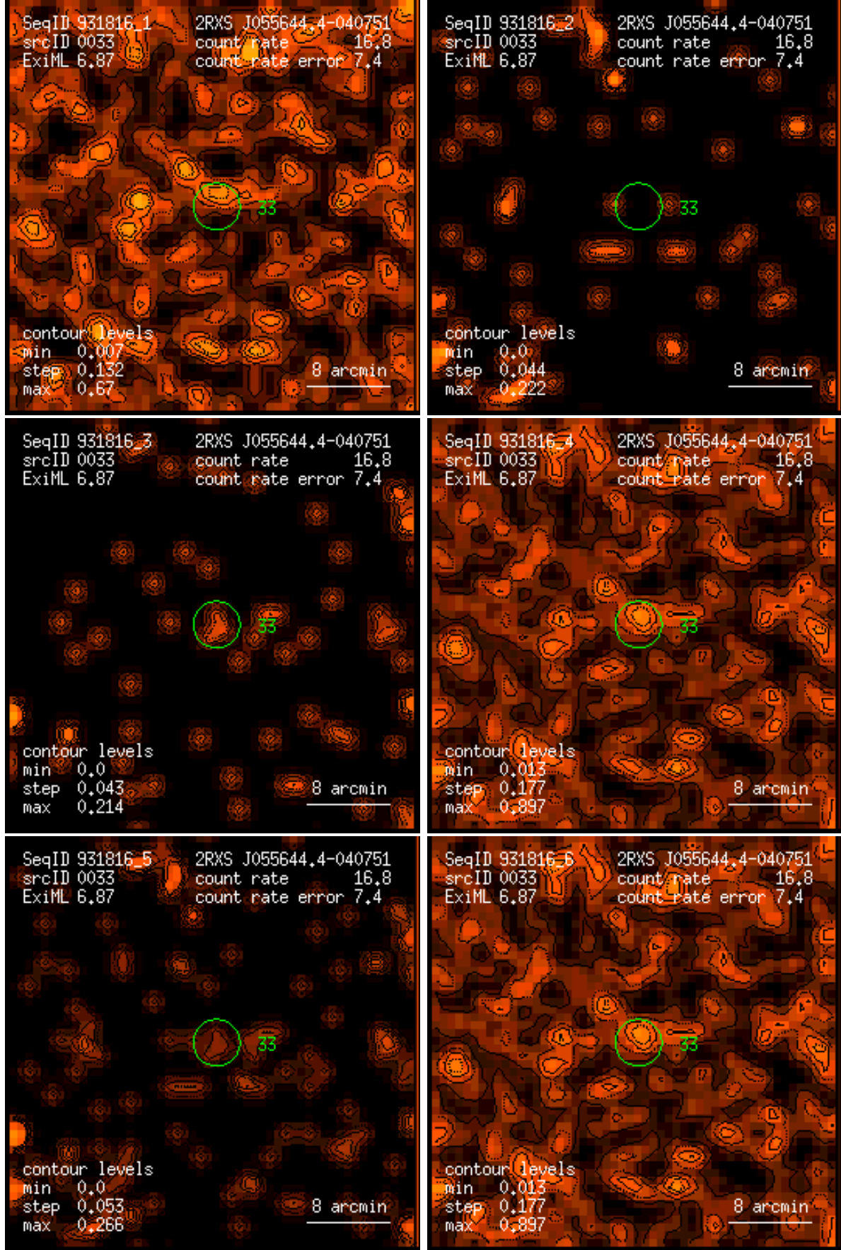
Figure 33: RASS 931816: detection 0033: band rate images, Gaussian filter: (1) PSPC channels 11 – 41, (2) 52 – 90, (3) 91 – 201, (4) 11 – 235, (5) 52 – 201, (6) 11 – 201. Broad band rates in counts/ks. Band rate contour levels in counts/ks/arcmin 2 .
