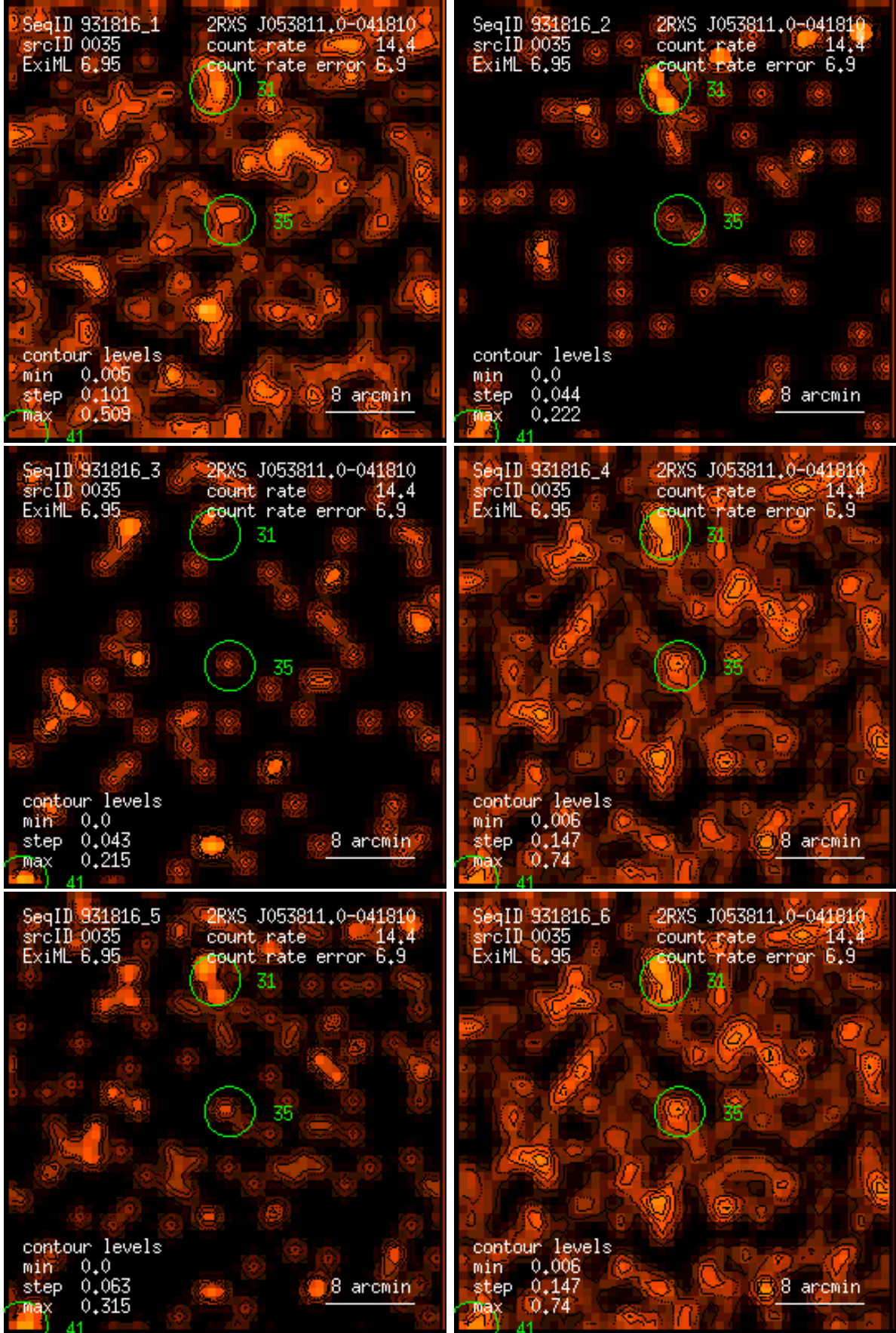
Figure 35: RASS 931816: detection 0035: band rate images, Gaussian filter: (1) PSPC channels 11 – 41, (2) 52 – 90, (3) 91 – 201, (4) 11 – 235, (5) 52 – 201, (6) 11 – 201. Broad band rates in counts/ks. Band rate contour levels in counts/ks/arcmin 2 .
