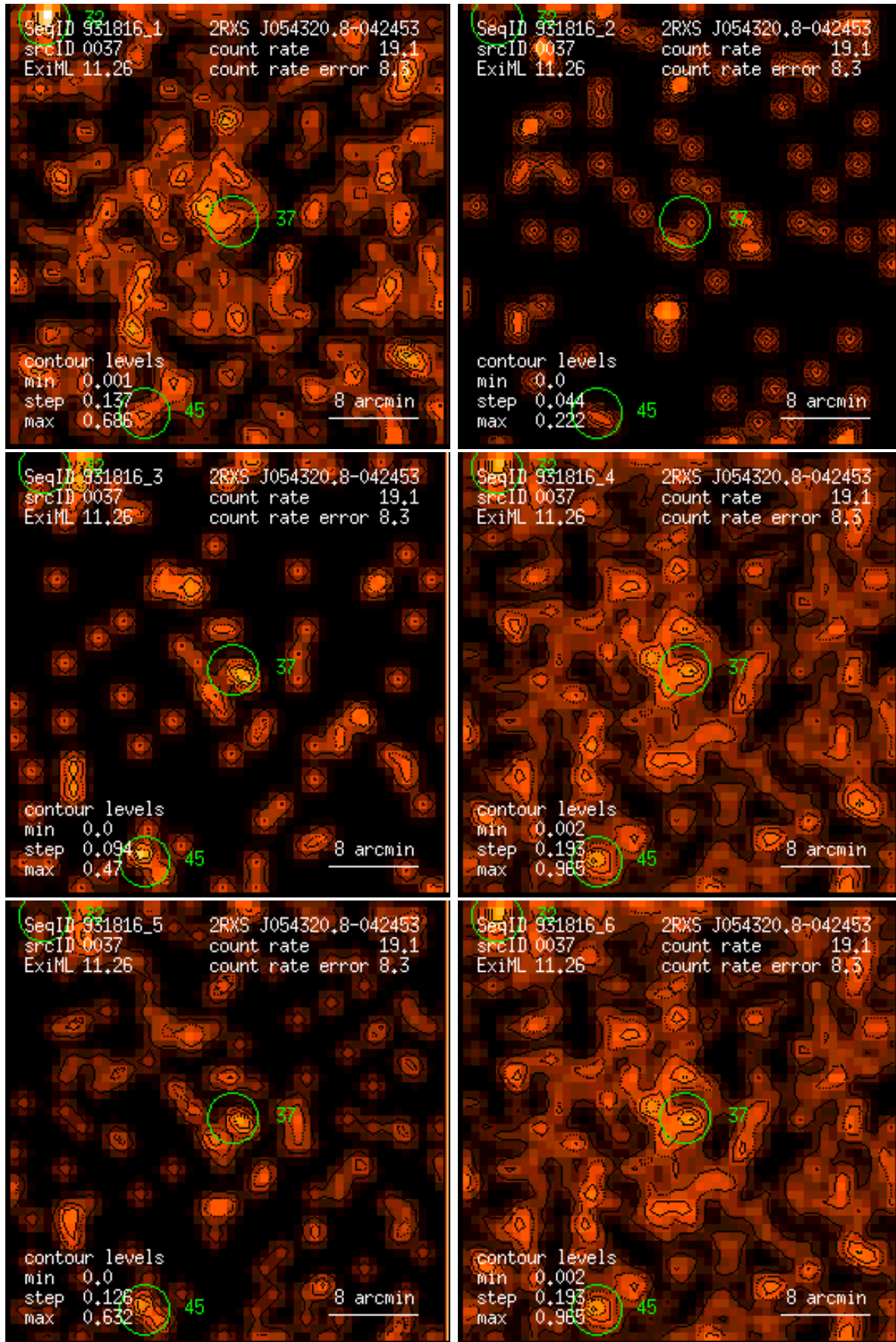
Figure 37: RASS 931816: detection 0037: band rate images, Gaussian filter: (1) PSPC channels 11 – 41, (2) 52 – 90, (3) 91 – 201, (4) 11 – 235, (5) 52 – 201, (6) 11 – 201. Broad band rates in counts/ks. Band rate contour levels in counts/ks/arcmin 2 .
