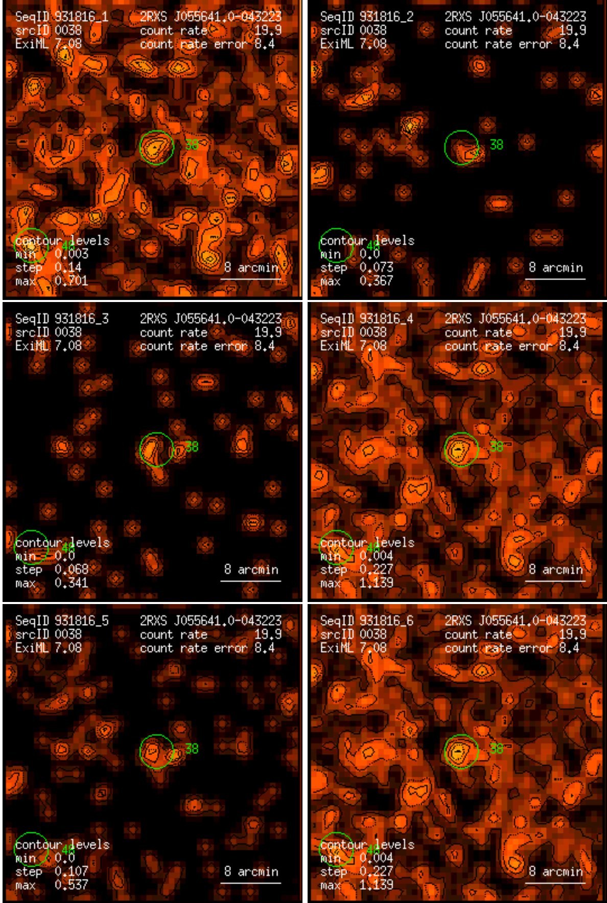
Figure 38: RASS 931816: detection 0038: band rate images, Gaussian filter: (1) PSPC channels 11 – 41, (2) 52 – 90, (3) 91 – 201, (4) 11 – 235, (5) 52 – 201, (6) 11 – 201. Broad band rates in counts/ks. Band rate contour levels in counts/ks/arcmin 2 .
