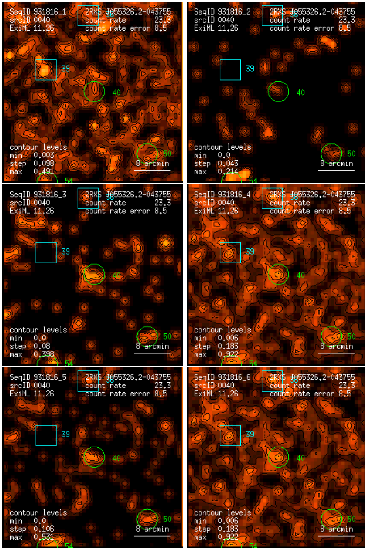
Figure 40: RASS 931816: detection 0040: band rate images, Gaussian filter: (1) PSPC channels 11 – 41, (2) 52 – 90, (3) 91 – 201, (4) 11 – 235, (5) 52 – 201, (6) 11 – 201. Broad band rates in counts/ks. Band rate contour levels in counts/ks/arcmin 2 .
