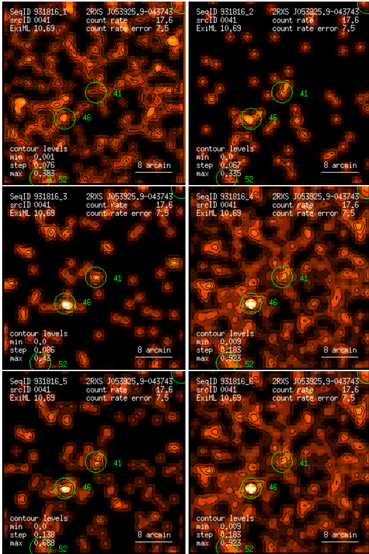
Figure 41: RASS 931816: detection 0041: band rate images, Gaussian filter: (1) PSPC channels 11 – 41, (2) 52 – 90, (3) 91 – 201, (4) 11 – 235, (5) 52 – 201, (6) 11 – 201. Broad band rates in counts/ks. Band rate contour levels in counts/ks/arcmin 2 .
