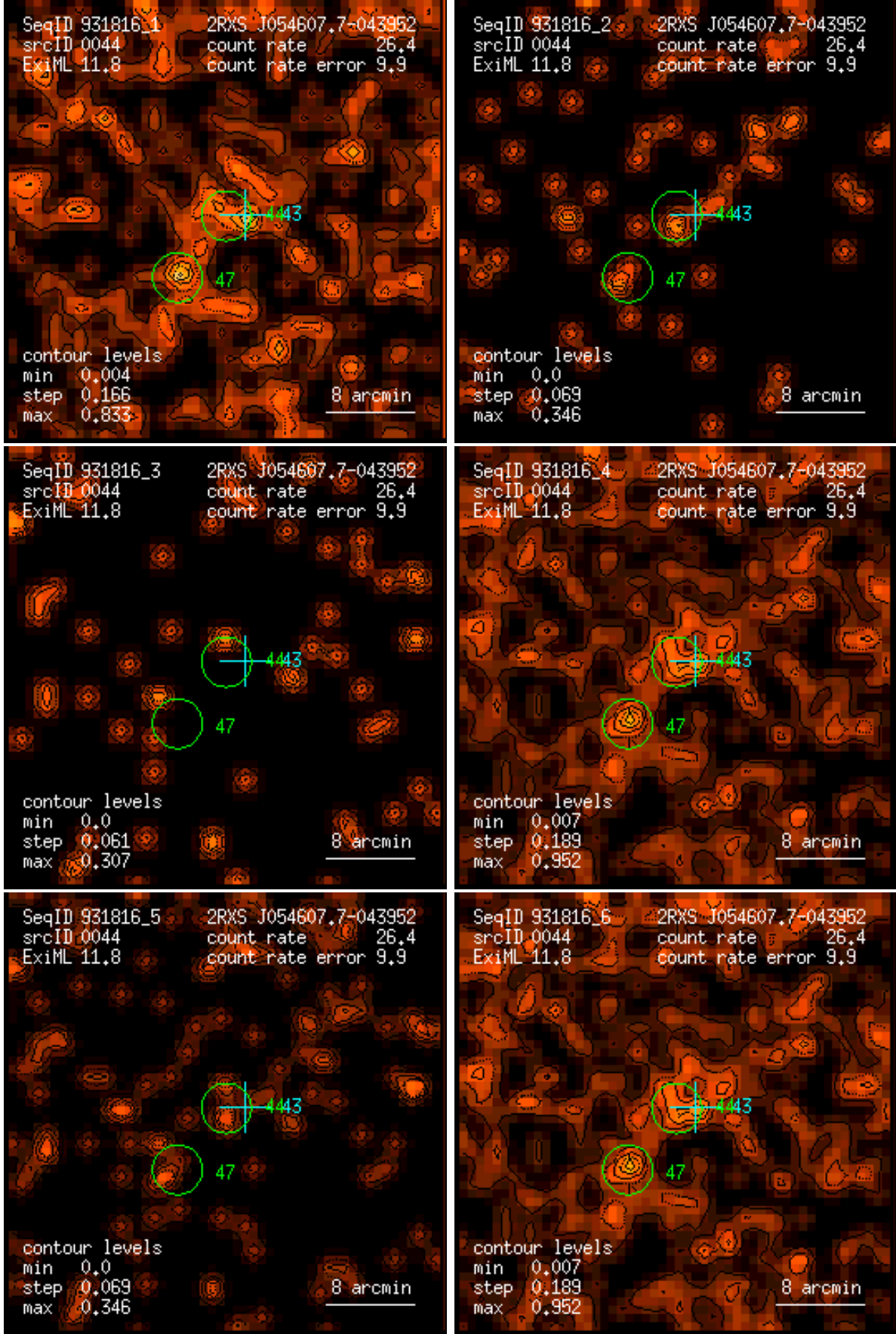
Figure 44: RASS 931816: detection 0044: band rate images, Gaussian filter: (1) PSPC channels 11 – 41, (2) 52 – 90, (3) 91 – 201, (4) 11 – 235, (5) 52 – 201, (6) 11 – 201. Broad band rates in counts/ks. Band rate contour levels in counts/ks/arcmin 2 .
