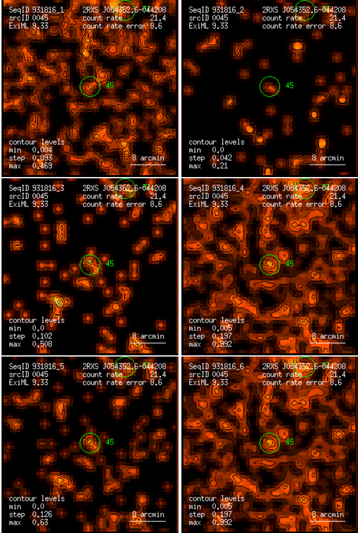
Figure 45: RASS 931816: detection 0045: band rate images, Gaussian filter: (1) PSPC channels 11 – 41, (2) 52 – 90, (3) 91 – 201, (4) 11 – 235, (5) 52 – 201, (6) 11 – 201. Broad band rates in counts/ks. Band rate contour levels in counts/ks/arcmin 2 .
