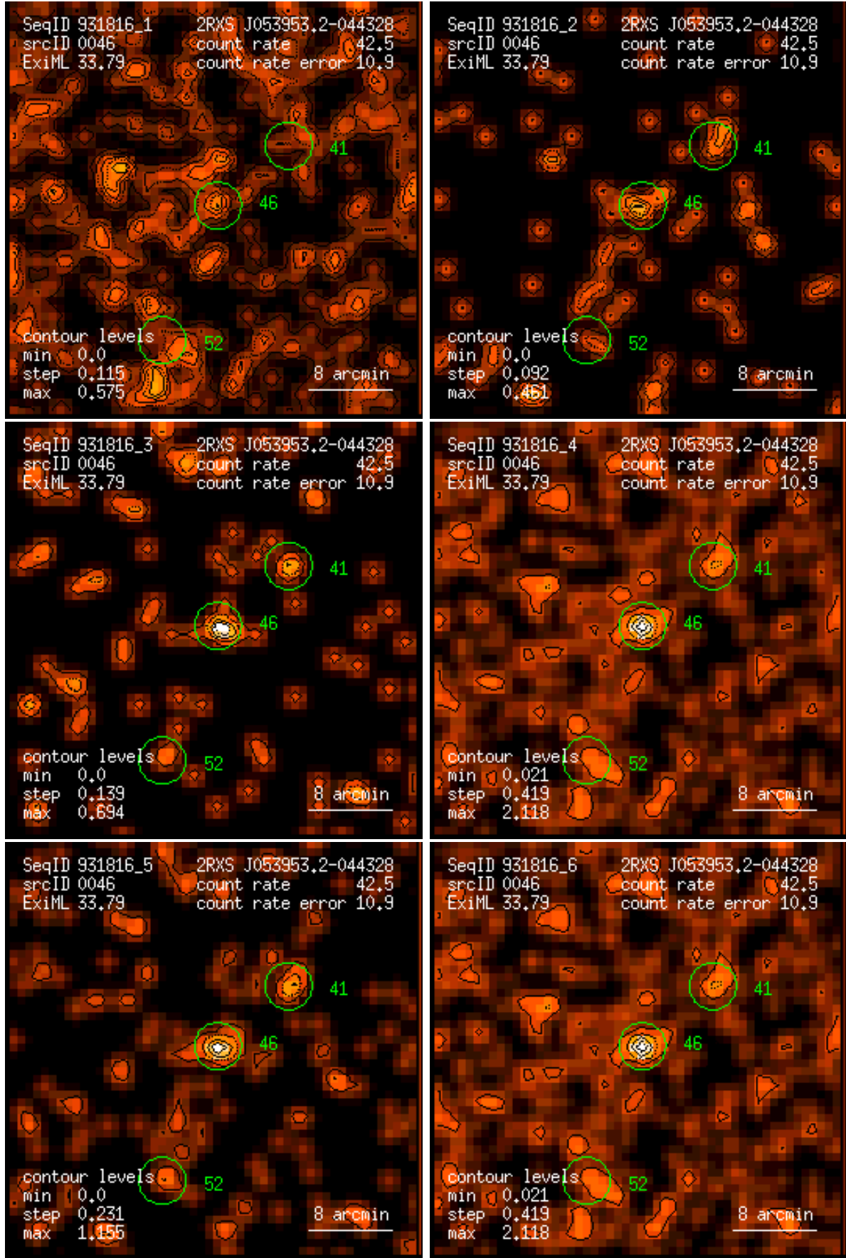
Figure 46: RASS 931816: detection 0046: band rate images, Gaussian filter: (1) PSPC channels 11 – 41, (2) 52 – 90, (3) 91 – 201, (4) 11 – 235, (5) 52 – 201, (6) 11 – 201. Broad band rates in counts/ks. Band rate contour levels in counts/ks/arcmin 2 .
