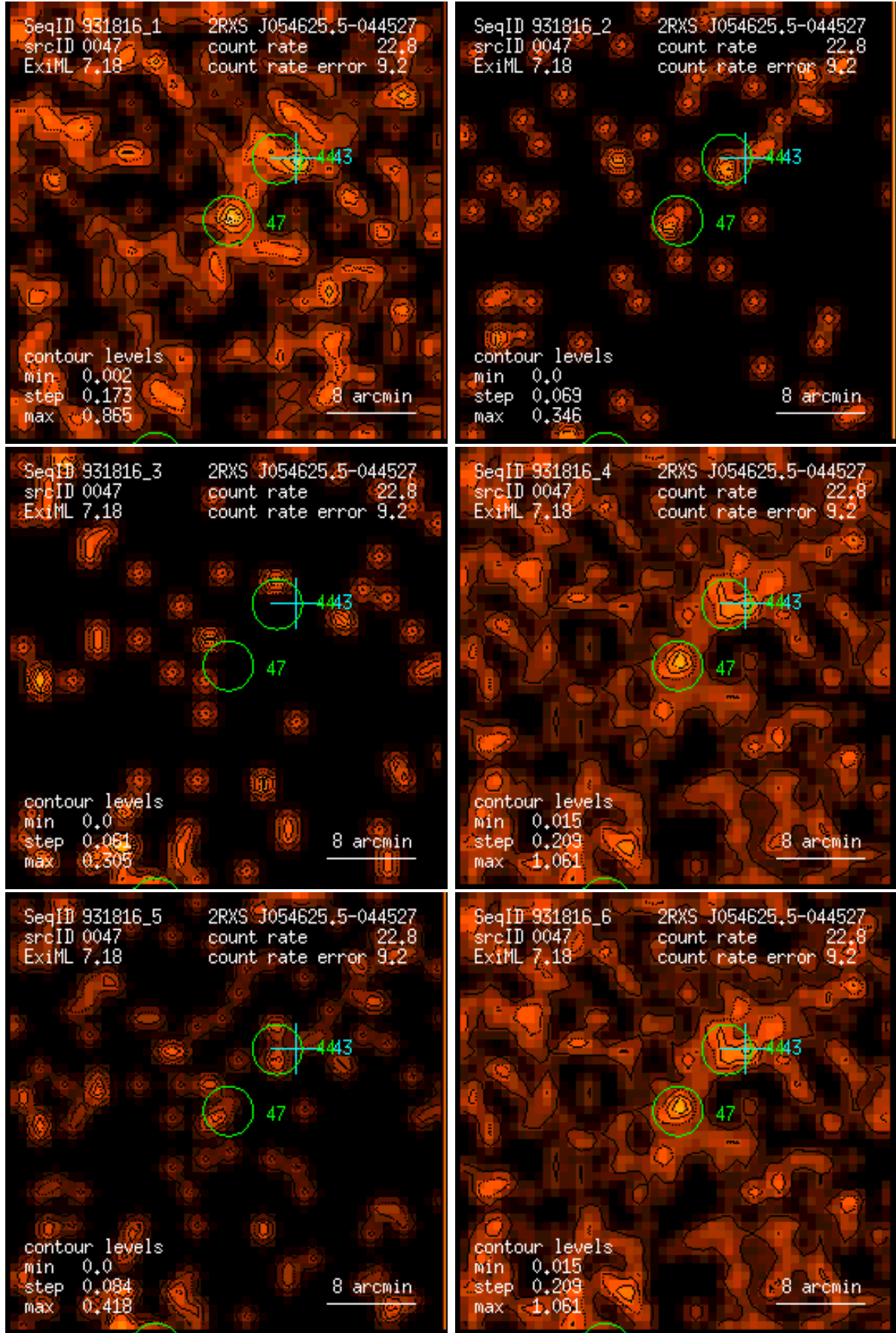
Figure 47: RASS 931816: detection 0047: band rate images, Gaussian filter: (1) PSPC channels 11 – 41, (2) 52 – 90, (3) 91 – 201, (4) 11 – 235, (5) 52 – 201, (6) 11 – 201. Broad band rates in counts/ks. Band rate contour levels in counts/ks/arcmin 2 .
