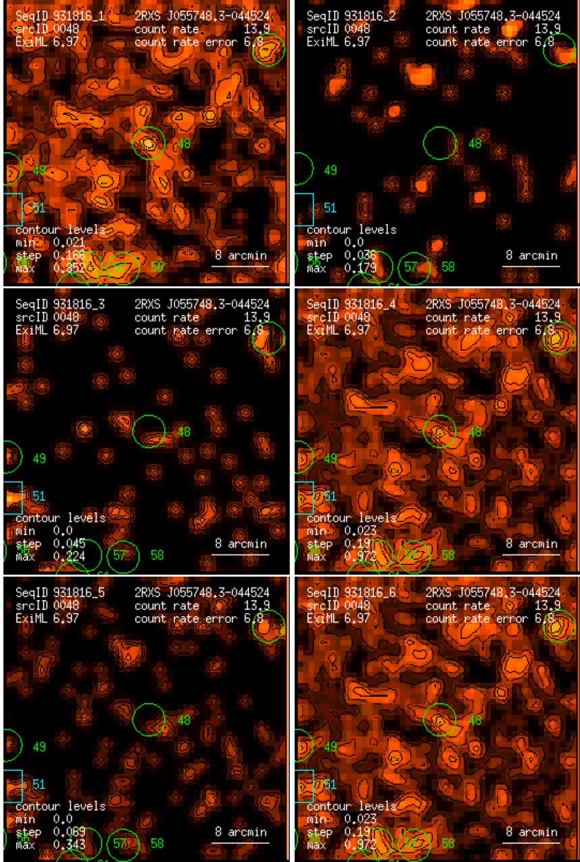
Figure 48: RASS 931816: detection 0048: band rate images, Gaussian filter: (1) PSPC channels 11 – 41, (2) 52 – 90, (3) 91 – 201, (4) 11 – 235, (5) 52 – 201, (6) 11 – 201. Broad band rates in counts/ks. Band rate contour levels in counts/ks/arcmin 2 .
