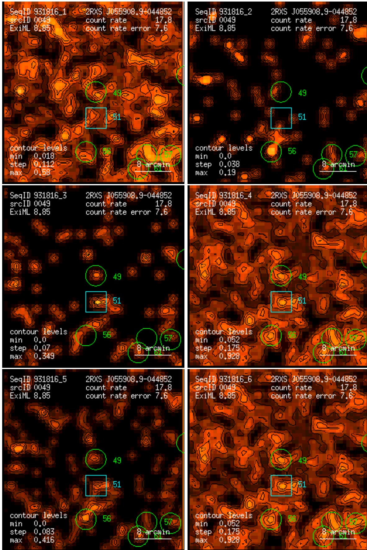
Figure 49: RASS 931816: detection 0049: band rate images, Gaussian filter: (1) PSPC channels 11 – 41, (2) 52 – 90, (3) 91 – 201, (4) 11 – 235, (5) 52 – 201, (6) 11 – 201. Broad band rates in counts/ks. Band rate contour levels in counts/ks/arcmin 2 .
