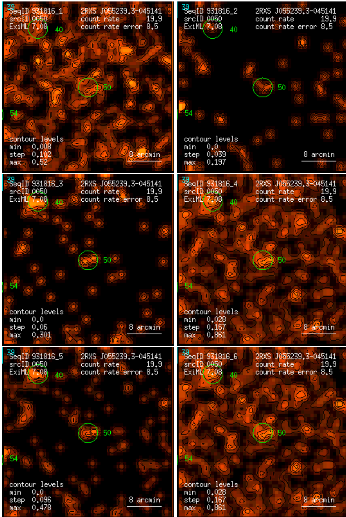
Figure 50: RASS 931816: detection 0050: band rate images, Gaussian filter: (1) PSPC channels 11 – 41, (2) 52 – 90, (3) 91 – 201, (4) 11 – 235, (5) 52 – 201, (6) 11 – 201. Broad band rates in counts/ks. Band rate contour levels in counts/ks/arcmin 2 .
