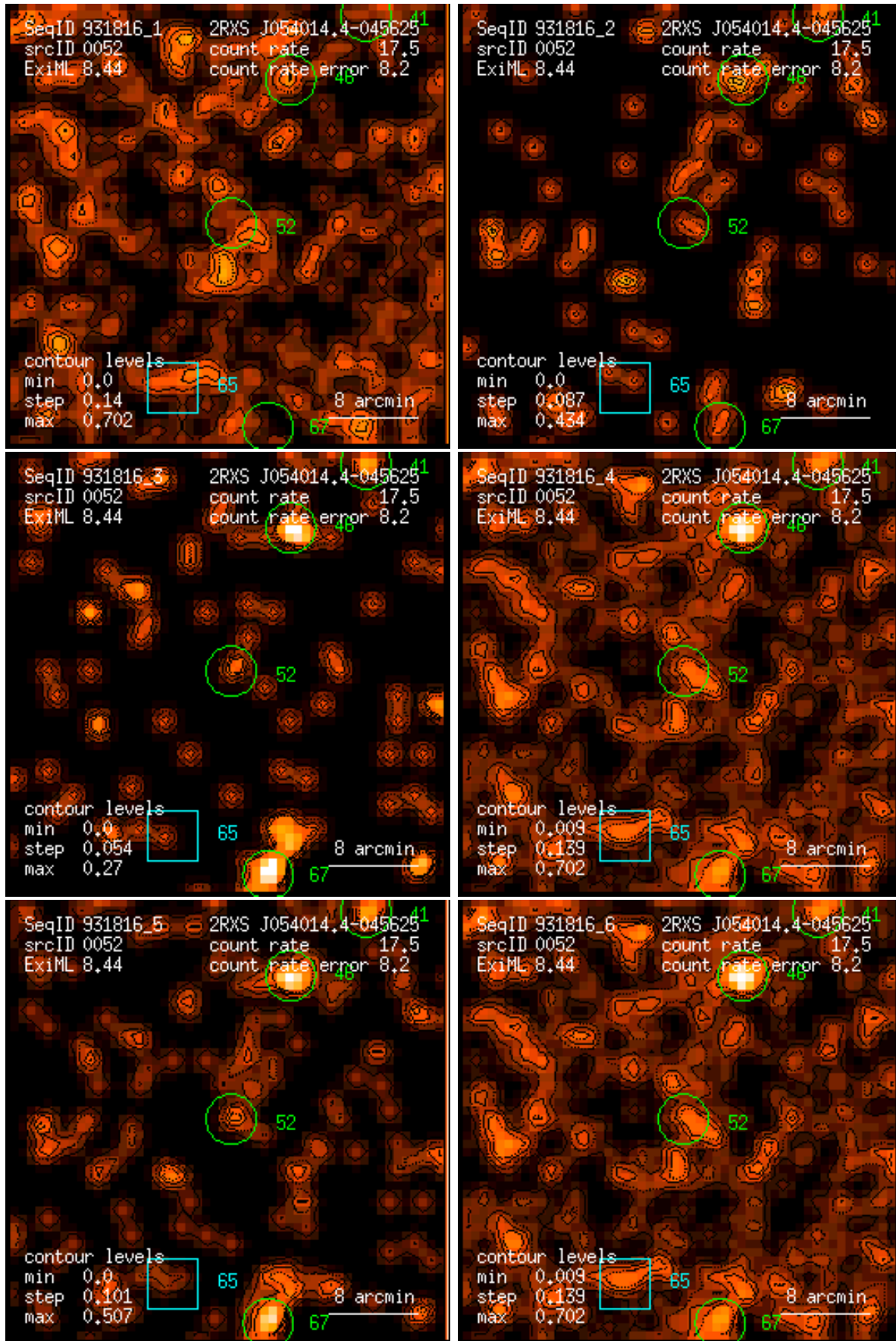
Figure 52: RASS 931816: detection 0052: band rate images, Gaussian filter: (1) PSPC channels 11 – 41, (2) 52 – 90, (3) 91 – 201, (4) 11 – 235, (5) 52 – 201, (6) 11 – 201. Broad band rates in counts/ks. Band rate contour levels in counts/ks/arcmin 2 .
