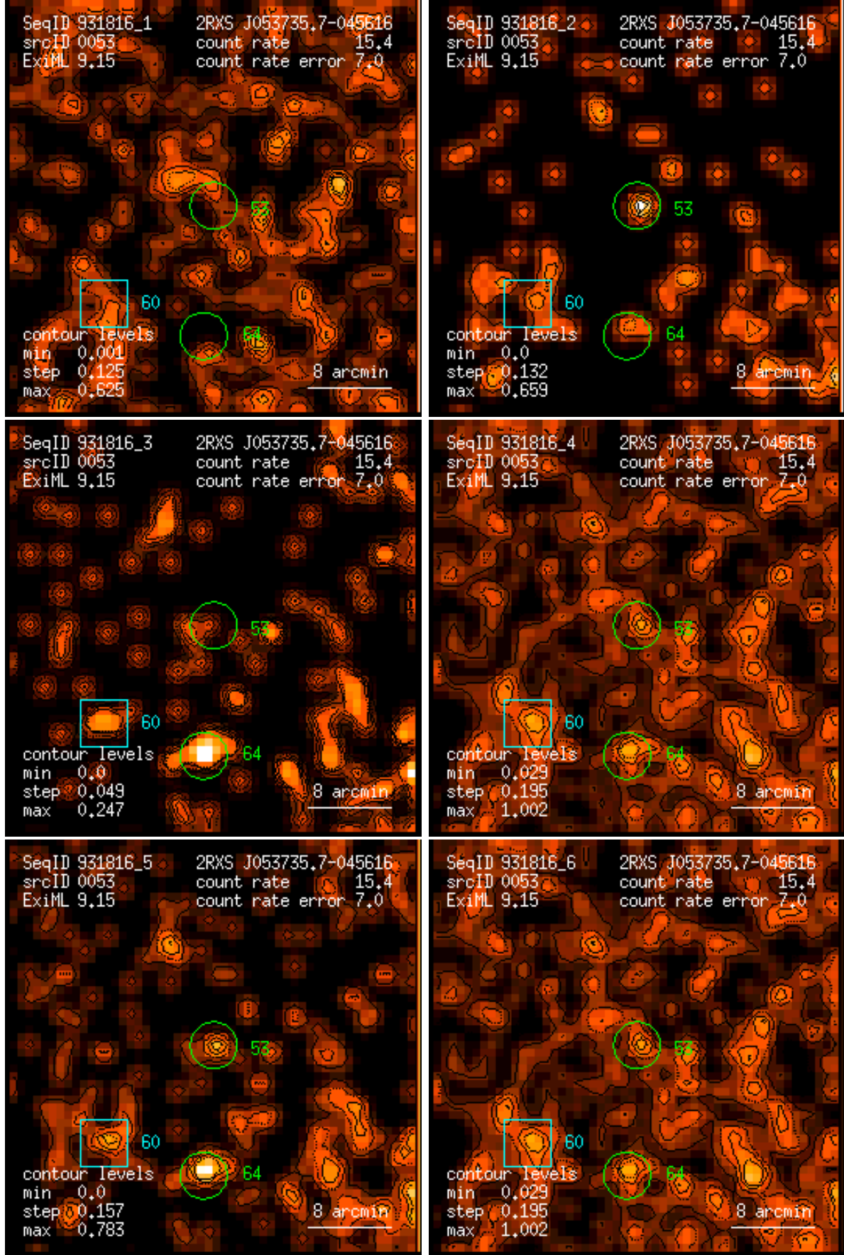
Figure 53: RASS 931816: detection 0053: band rate images, Gaussian filter: (1) PSPC channels 11 – 41, (2) 52 – 90, (3) 91 – 201, (4) 11 – 235, (5) 52 – 201, (6) 11 – 201. Broad band rates in counts/ks. Band rate contour levels in counts/ks/arcmin 2 .
