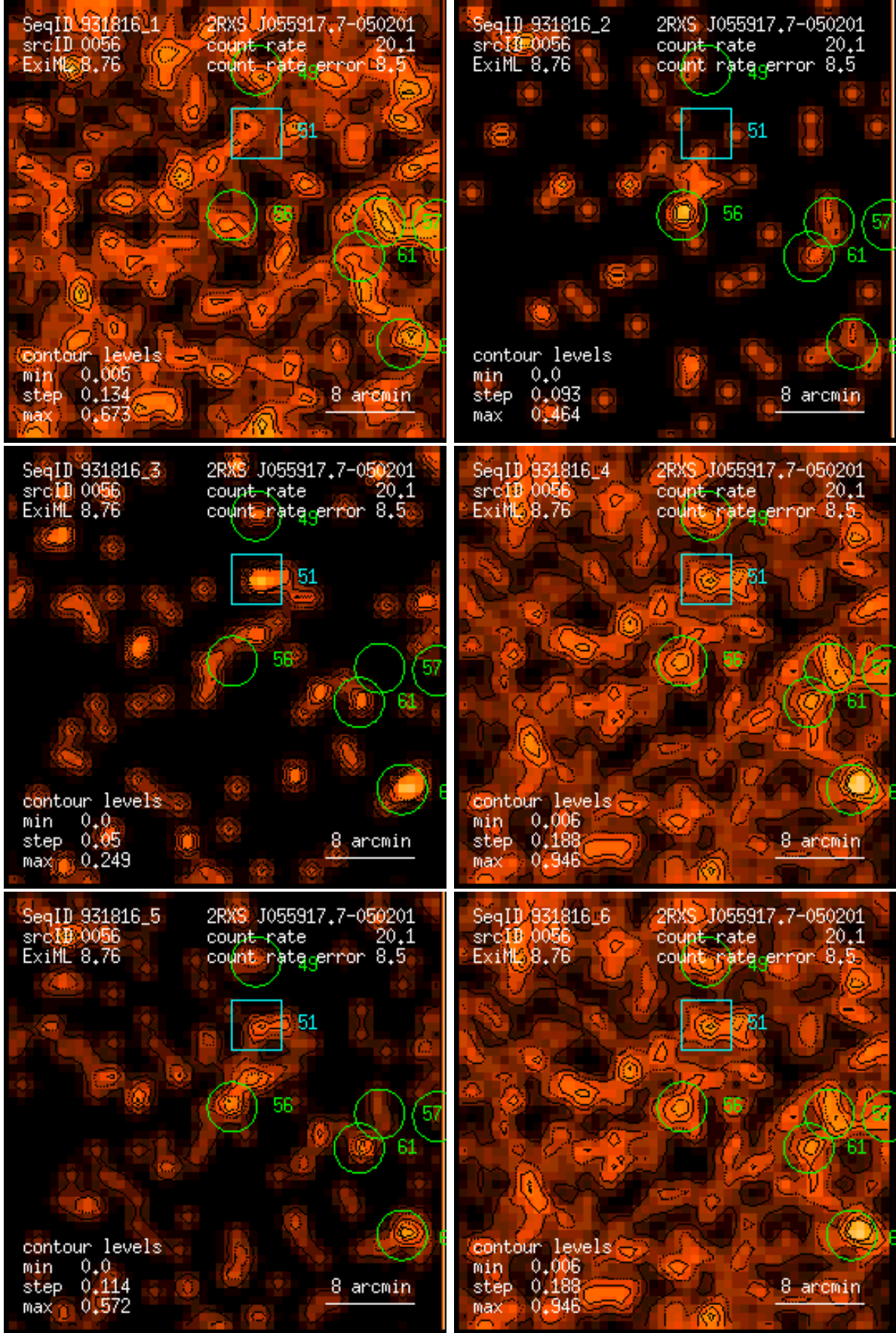
Figure 56: RASS 931816: detection 0056: band rate images, Gaussian filter: (1) PSPC channels 11 – 41, (2) 52 – 90, (3) 91 – 201, (4) 11 – 235, (5) 52 – 201, (6) 11 – 201. Broad band rates in counts/ks. Band rate contour levels in counts/ks/arcmin 2 .
