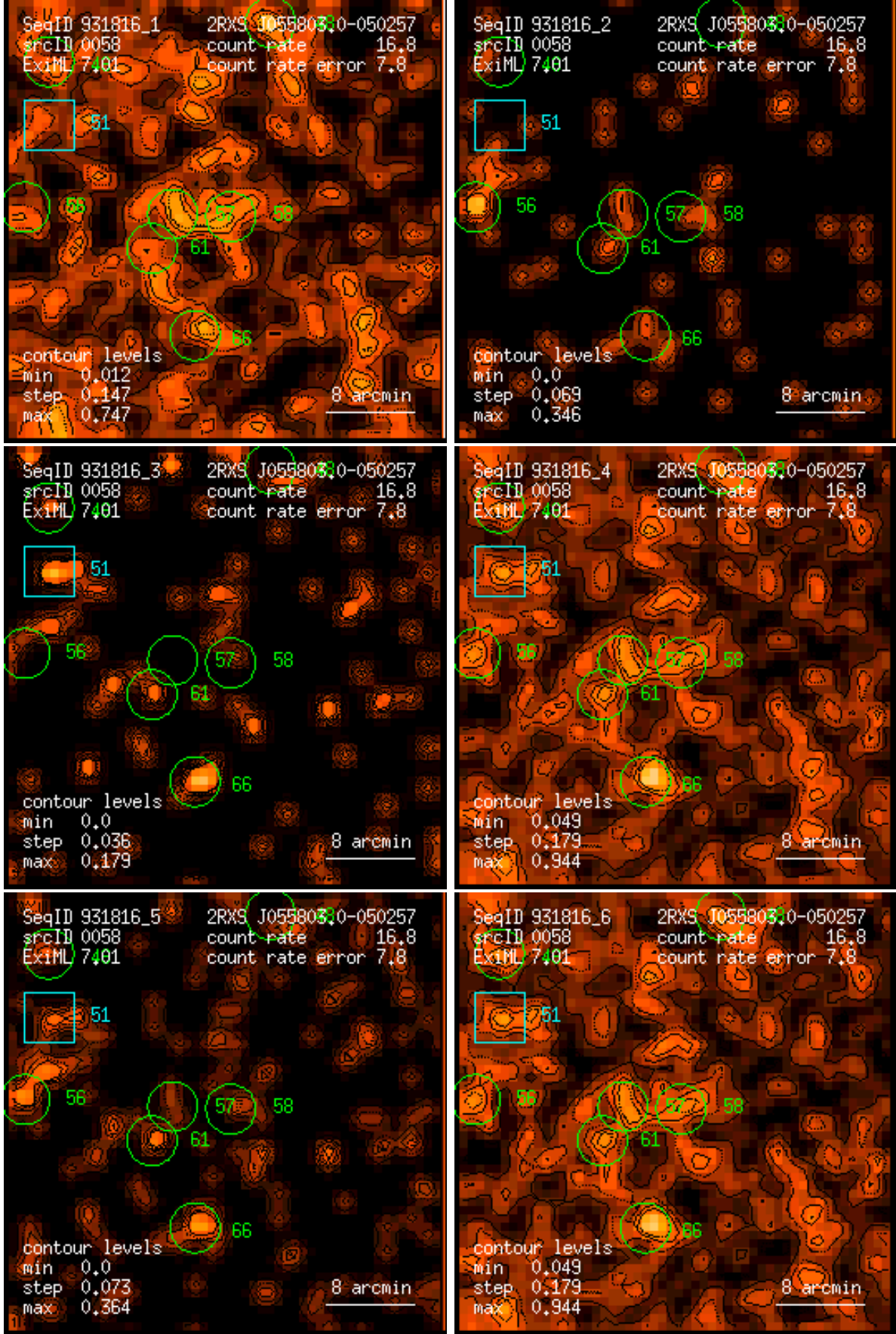
Figure 58: RASS 931816: detection 0058: band rate images, Gaussian filter: (1) PSPC channels 11 – 41, (2) 52 – 90, (3) 91 – 201, (4) 11 – 235, (5) 52 – 201, (6) 11 – 201. Broad band rates in counts/ks. Band rate contour levels in counts/ks/arcmin 2 .
