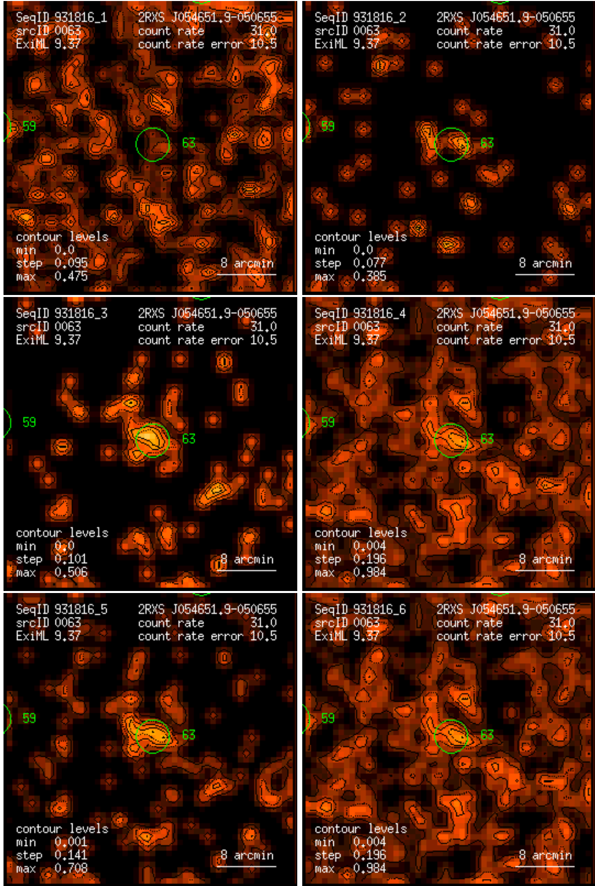
Figure 63: RASS 931816: detection 0063: band rate images, Gaussian filter: (1) PSPC channels 11 – 41, (2) 52 – 90, (3) 91 – 201, (4) 11 – 235, (5) 52 – 201, (6) 11 – 201. Broad band rates in counts/ks. Band rate contour levels in counts/ks/arcmin 2 .
