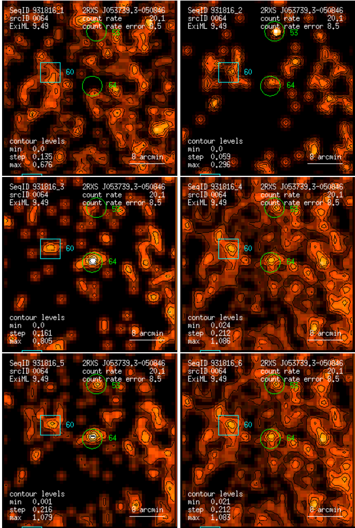
Figure 64: RASS 931816: detection 0064: band rate images, Gaussian filter: (1) PSPC channels 11 – 41, (2) 52 – 90, (3) 91 – 201, (4) 11 – 235, (5) 52 – 201, (6) 11 – 201. Broad band rates in counts/ks. Band rate contour levels in counts/ks/arcmin 2 .
