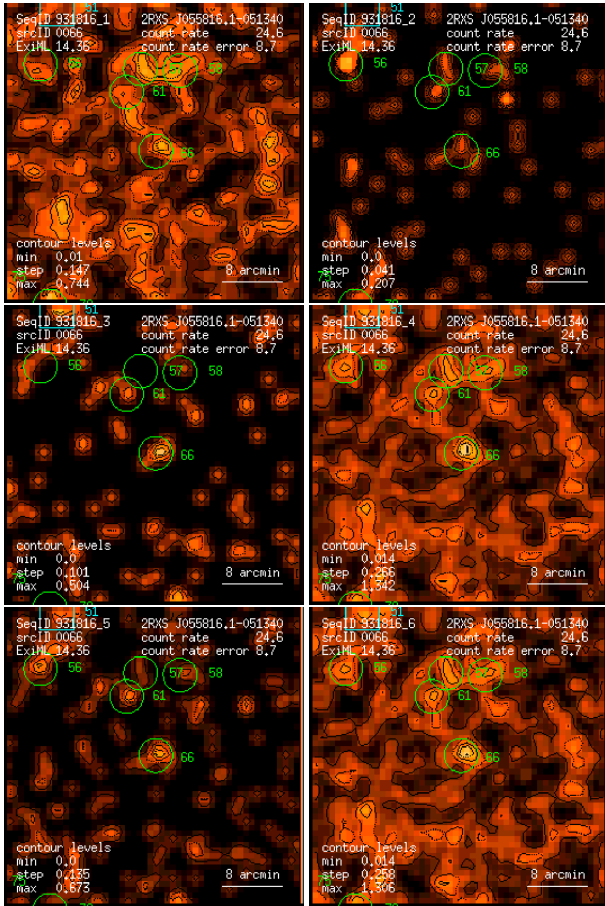
Figure 66: RASS 931816: detection 0066: band rate images, Gaussian filter: (1) PSPC channels 11 – 41, (2) 52 – 90, (3) 91 – 201, (4) 11 – 235, (5) 52 – 201, (6) 11 – 201. Broad band rates in counts/ks. Band rate contour levels in counts/ks/arcmin 2 .
