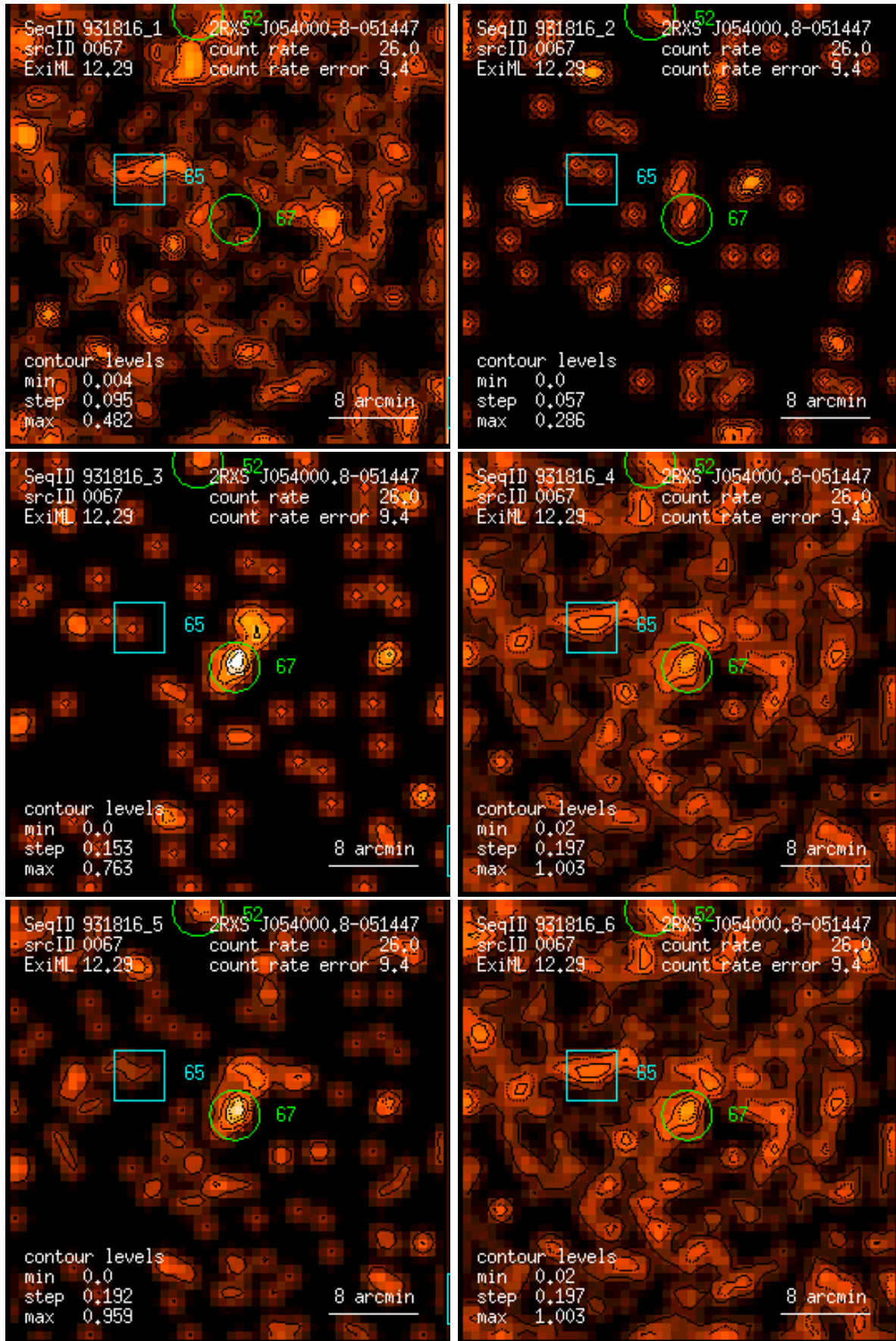
Figure 67: RASS 931816: detection 0067: band rate images, Gaussian filter: (1) PSPC channels 11 – 41, (2) 52 – 90, (3) 91 – 201, (4) 11 – 235, (5) 52 – 201, (6) 11 – 201. Broad band rates in counts/ks. Band rate contour levels in counts/ks/arcmin 2 .
