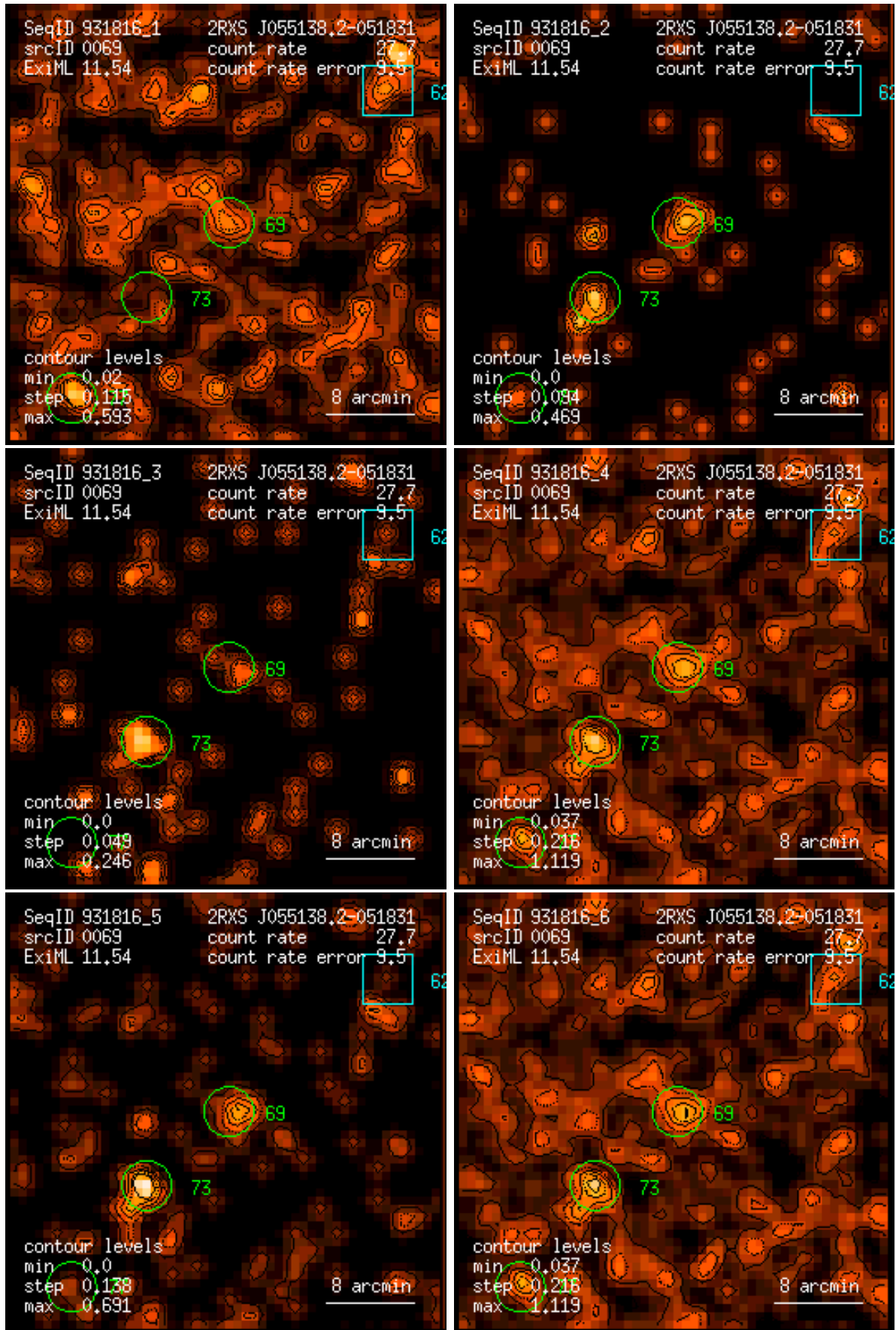
Figure 69: RASS 931816: detection 0069: band rate images, Gaussian filter: (1) PSPC channels 11 – 41, (2) 52 – 90, (3) 91 – 201, (4) 11 – 235, (5) 52 – 201, (6) 11 – 201. Broad band rates in counts/ks. Band rate contour levels in counts/ks/arcmin 2 .
