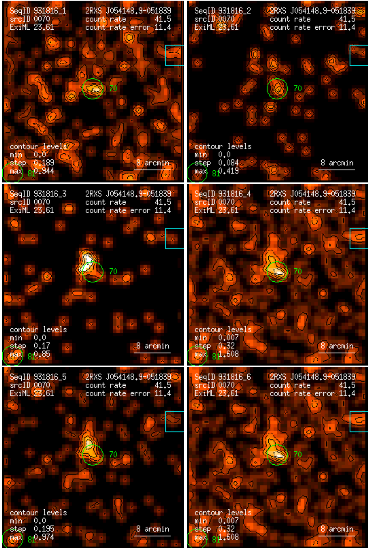
Figure 70: RASS 931816: detection 0070: band rate images, Gaussian filter: (1) PSPC channels 11 – 41, (2) 52 – 90, (3) 91 – 201, (4) 11 – 235, (5) 52 – 201, (6) 11 – 201. Broad band rates in counts/ks. Band rate contour levels in counts/ks/arcmin 2 .
