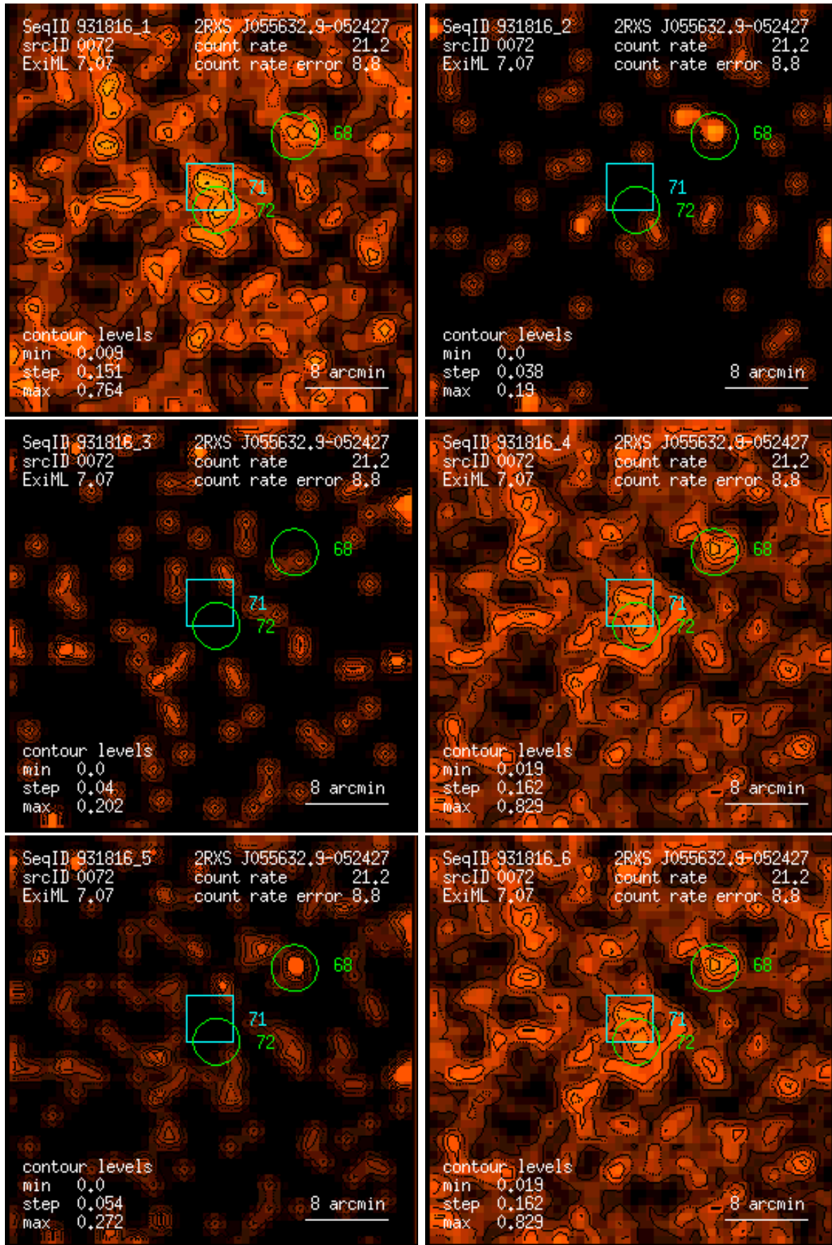
Figure 72: RASS 931816: detection 0072: band rate images, Gaussian filter: (1) PSPC channels 11 – 41, (2) 52 – 90, (3) 91 – 201, (4) 11 – 235, (5) 52 – 201, (6) 11 – 201. Broad band rates in counts/ks. Band rate contour levels in counts/ks/arcmin 2 .
