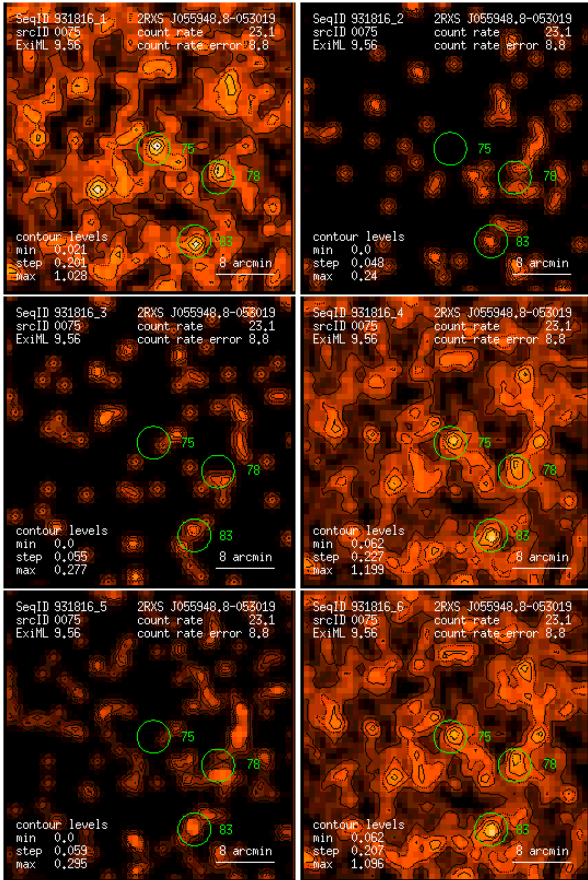
Figure 75: RASS 931816: detection 0075: band rate images, Gaussian filter: (1) PSPC channels 11 – 41, (2) 52 – 90, (3) 91 – 201, (4) 11 – 235, (5) 52 – 201, (6) 11 – 201. Broad band rates in counts/ks. Band rate contour levels in counts/ks/arcmin 2 .
