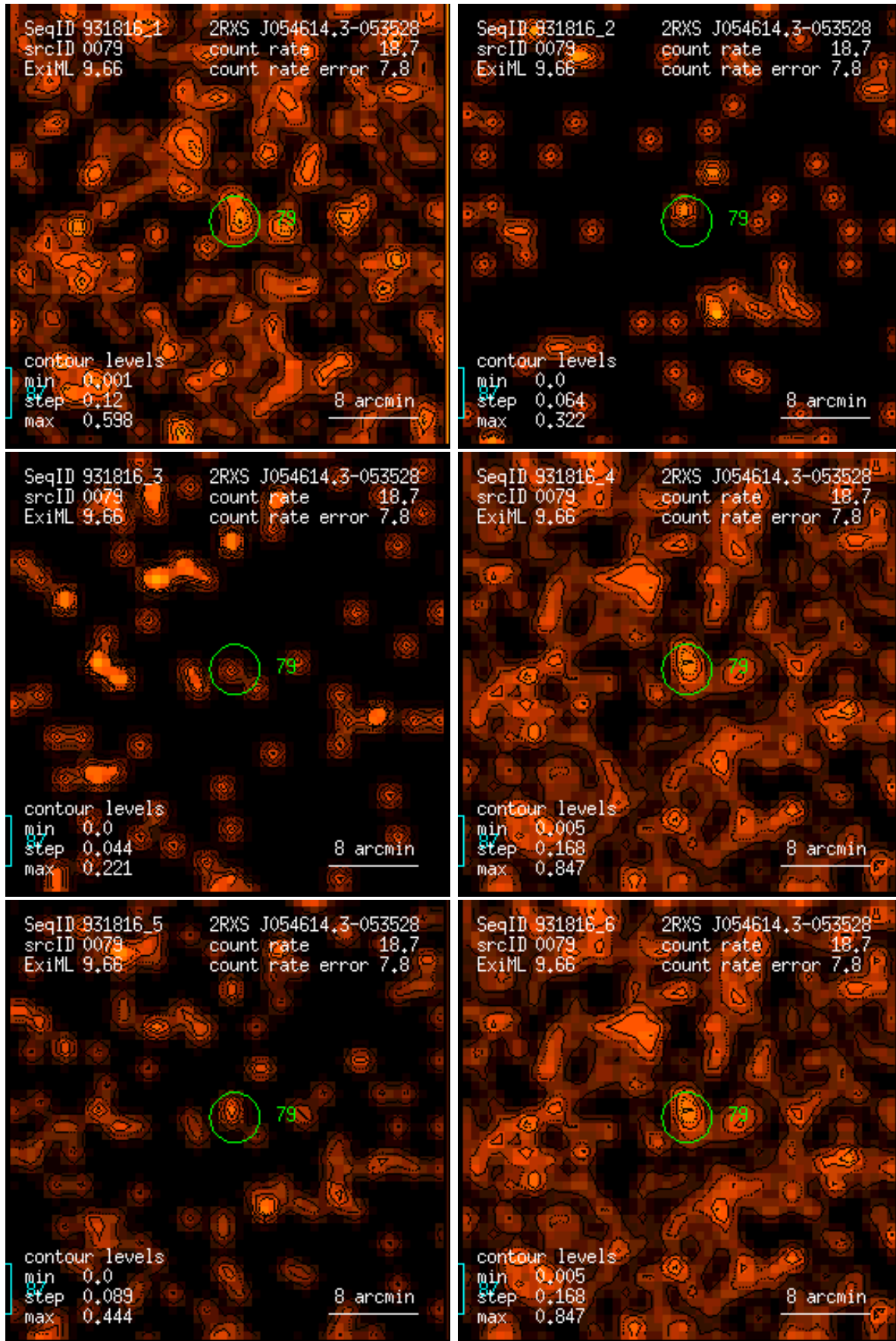
Figure 79: RASS 931816: detection 0079: band rate images, Gaussian filter: (1) PSPC channels 11 – 41, (2) 52 – 90, (3) 91 – 201, (4) 11 – 235, (5) 52 – 201, (6) 11 – 201. Broad band rates in counts/ks. Band rate contour levels in counts/ks/arcmin 2 .
