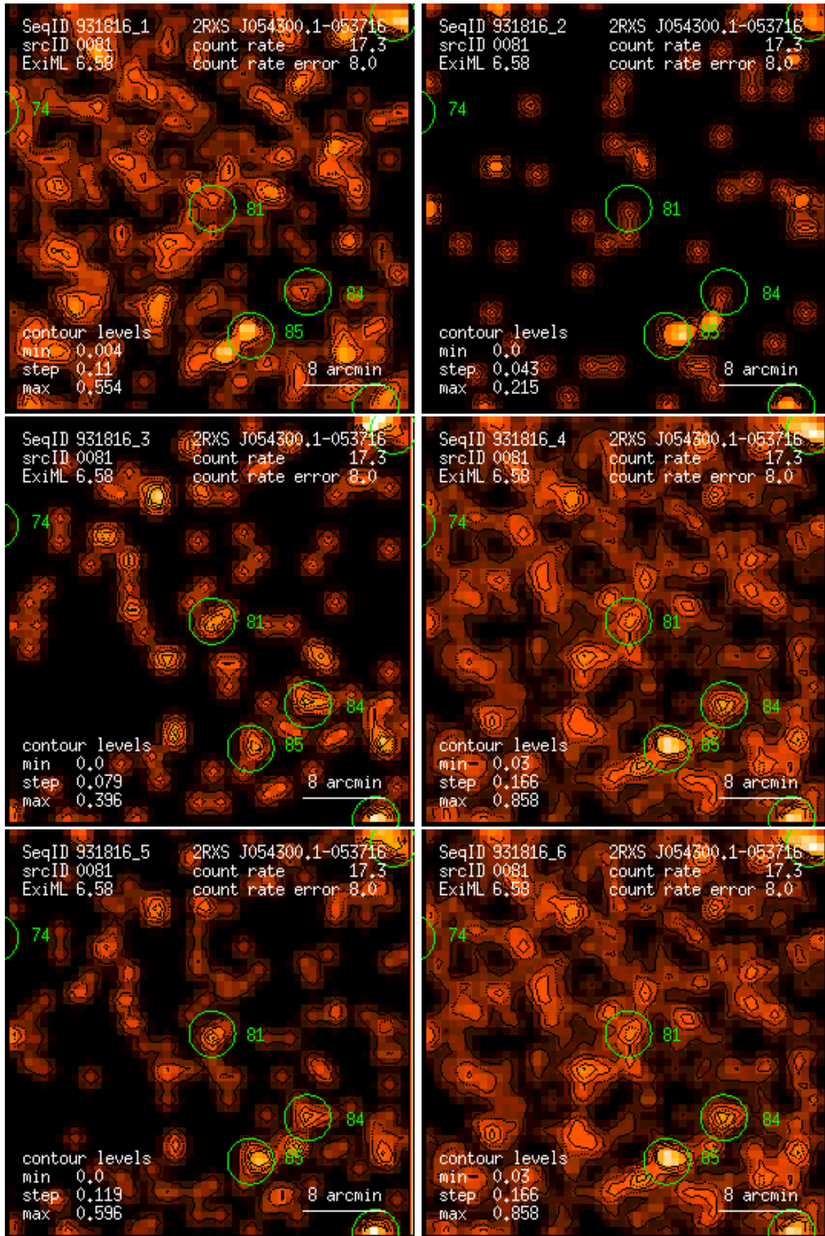
Figure 81: RASS 931816: detection 0081: band rate images, Gaussian filter: (1) PSPC channels 11 – 41, (2) 52 – 90, (3) 91 – 201, (4) 11 – 235, (5) 52 – 201, (6) 11 – 201. Broad band rates in counts/ks. Band rate contour levels in counts/ks/arcmin 2 .
