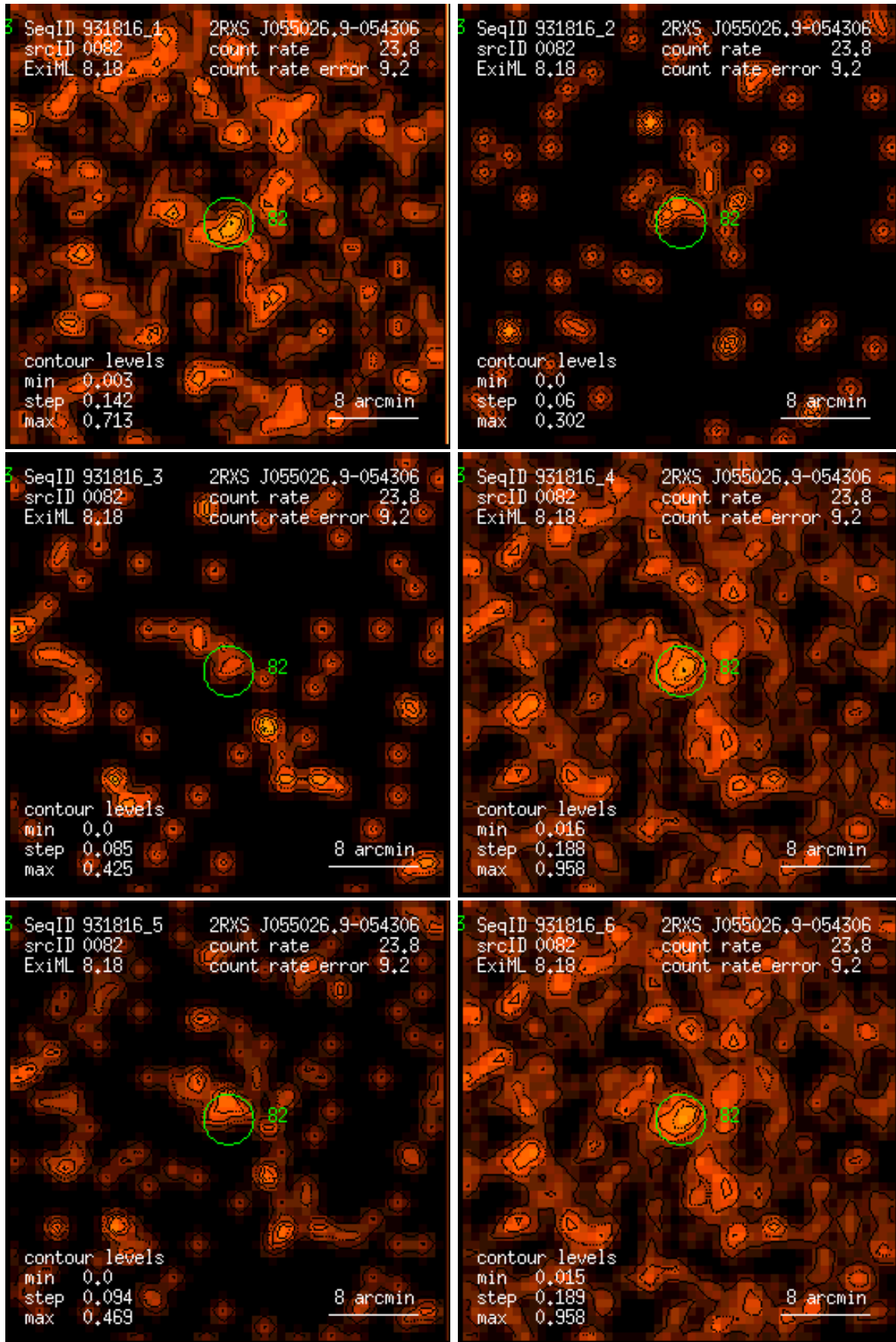
Figure 82: RASS 931816: detection 0082: band rate images, Gaussian filter: (1) PSPC channels 11 – 41, (2) 52 – 90, (3) 91 – 201, (4) 11 – 235, (5) 52 – 201, (6) 11 – 201. Broad band rates in counts/ks. Band rate contour levels in counts/ks/arcmin 2 .
