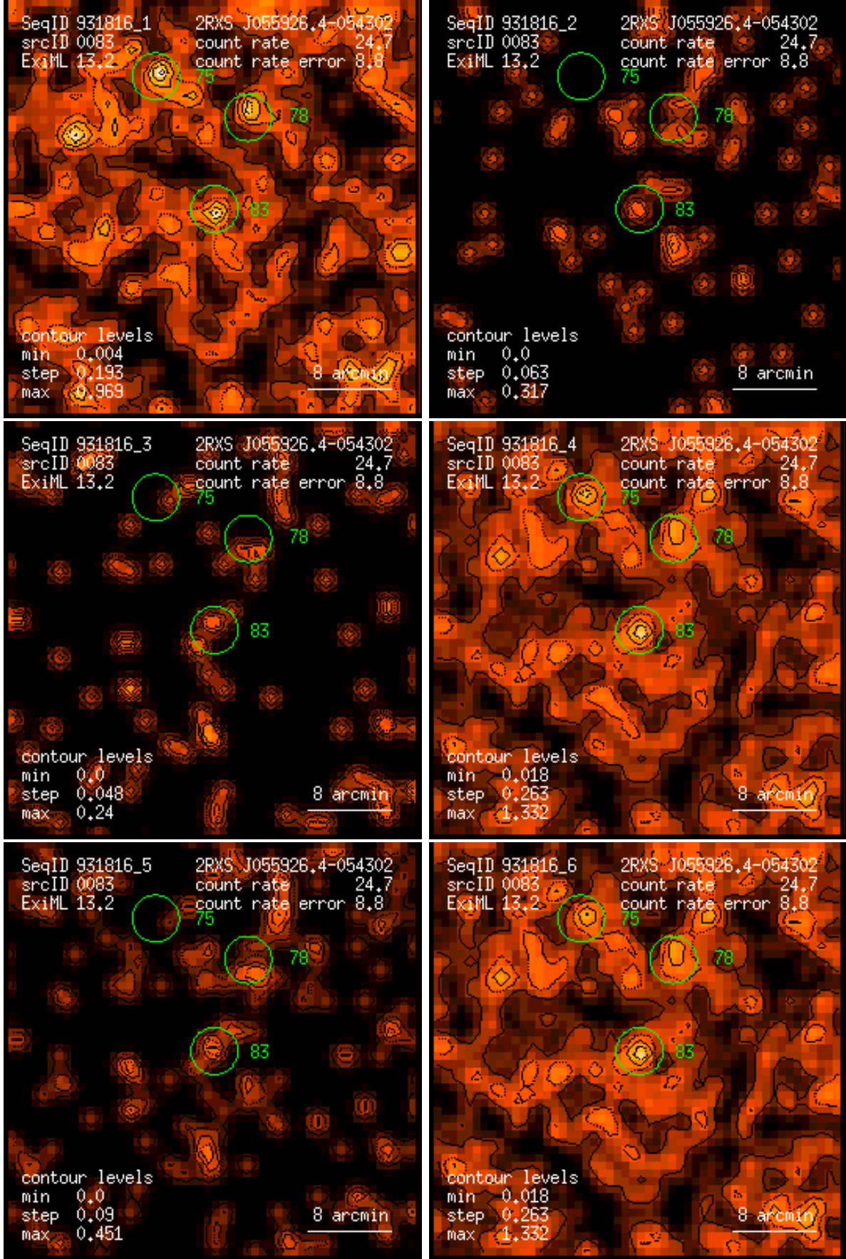
Figure 83: RASS 931816: detection 0083: band rate images, Gaussian filter: (1) PSPC channels 11 – 41, (2) 52 – 90, (3) 91 – 201, (4) 11 – 235, (5) 52 – 201, (6) 11 – 201. Broad band rates in counts/ks. Band rate contour levels in counts/ks/arcmin 2 .
