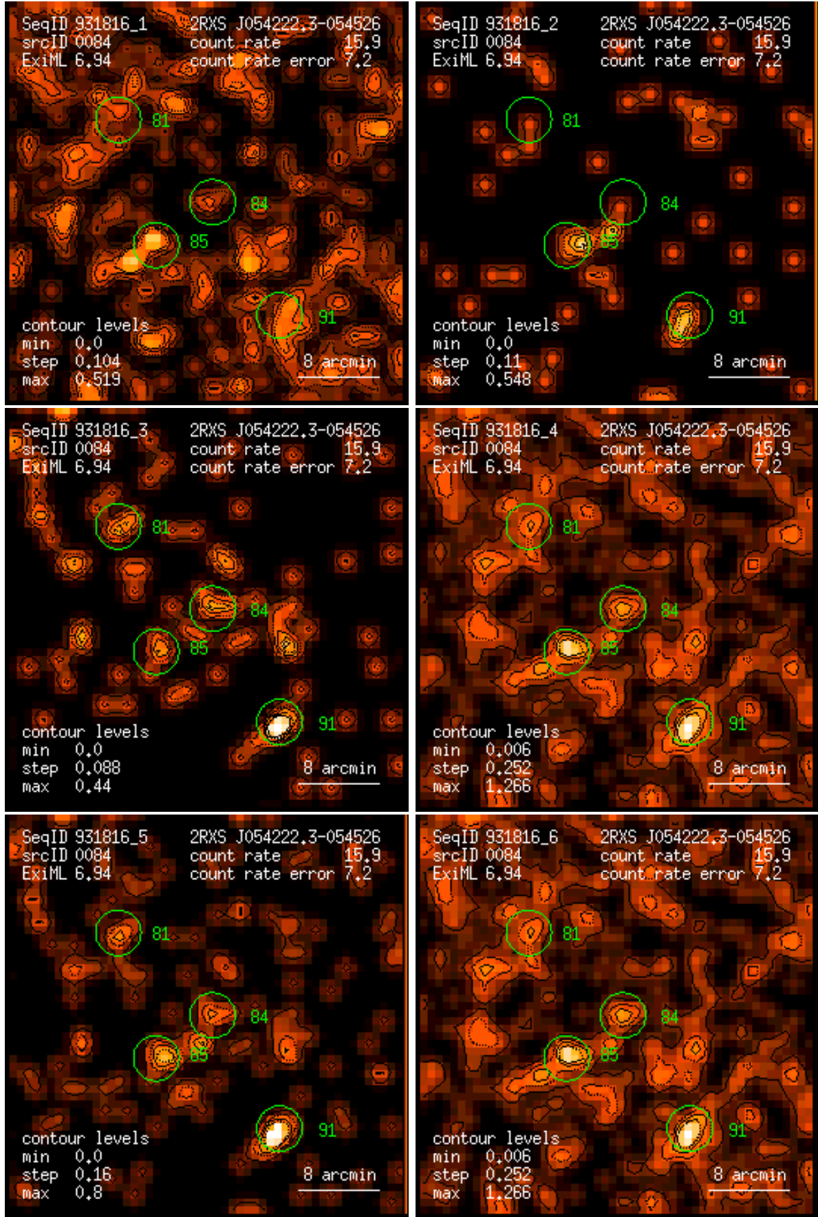
Figure 84: RASS 931816: detection 0084: band rate images, Gaussian filter: (1) PSPC channels 11 – 41, (2) 52 – 90, (3) 91 – 201, (4) 11 – 235, (5) 52 – 201, (6) 11 – 201. Broad band rates in counts/ks. Band rate contour levels in counts/ks/arcmin 2 .
