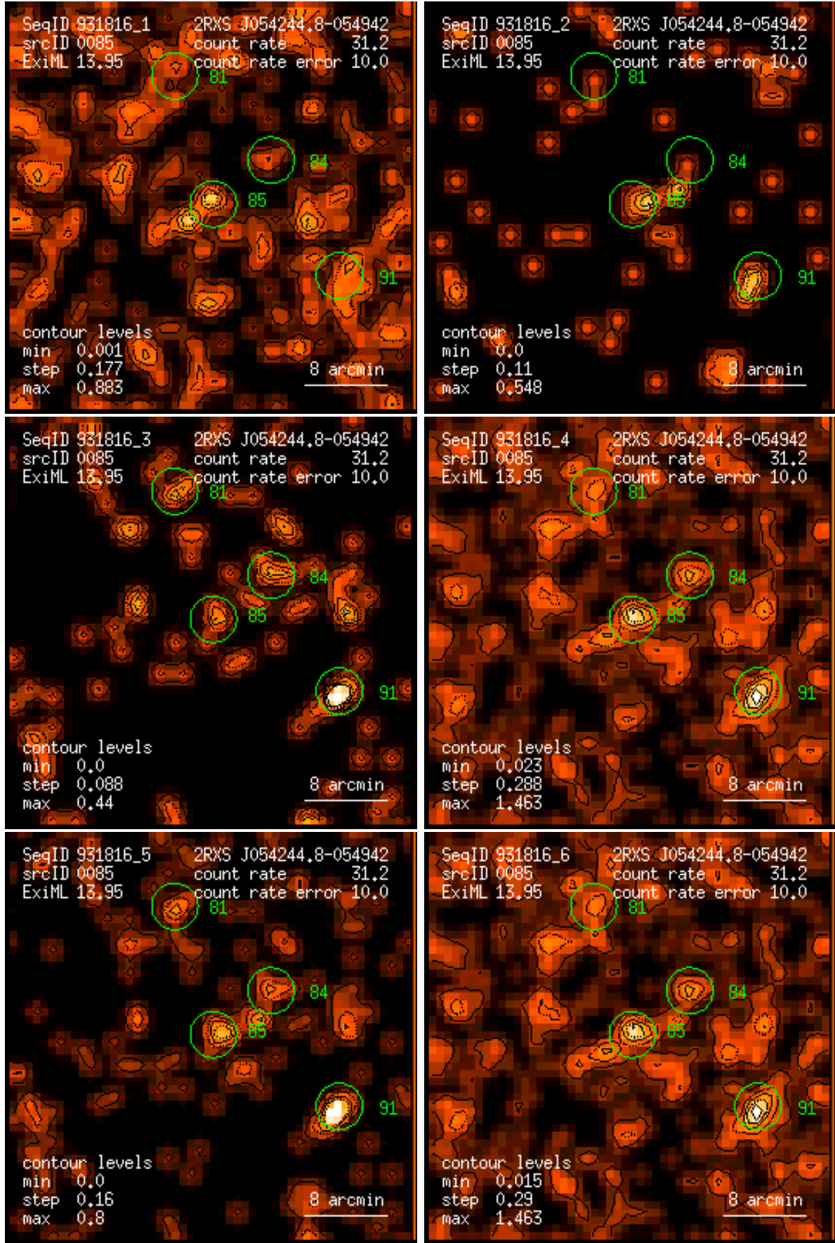
Figure 85: RASS 931816: detection 0085: band rate images, Gaussian filter: (1) PSPC channels 11 – 41, (2) 52 – 90, (3) 91 – 201, (4) 11 – 235, (5) 52 – 201, (6) 11 – 201. Broad band rates in counts/ks. Band rate contour levels in counts/ks/arcmin 2 .
