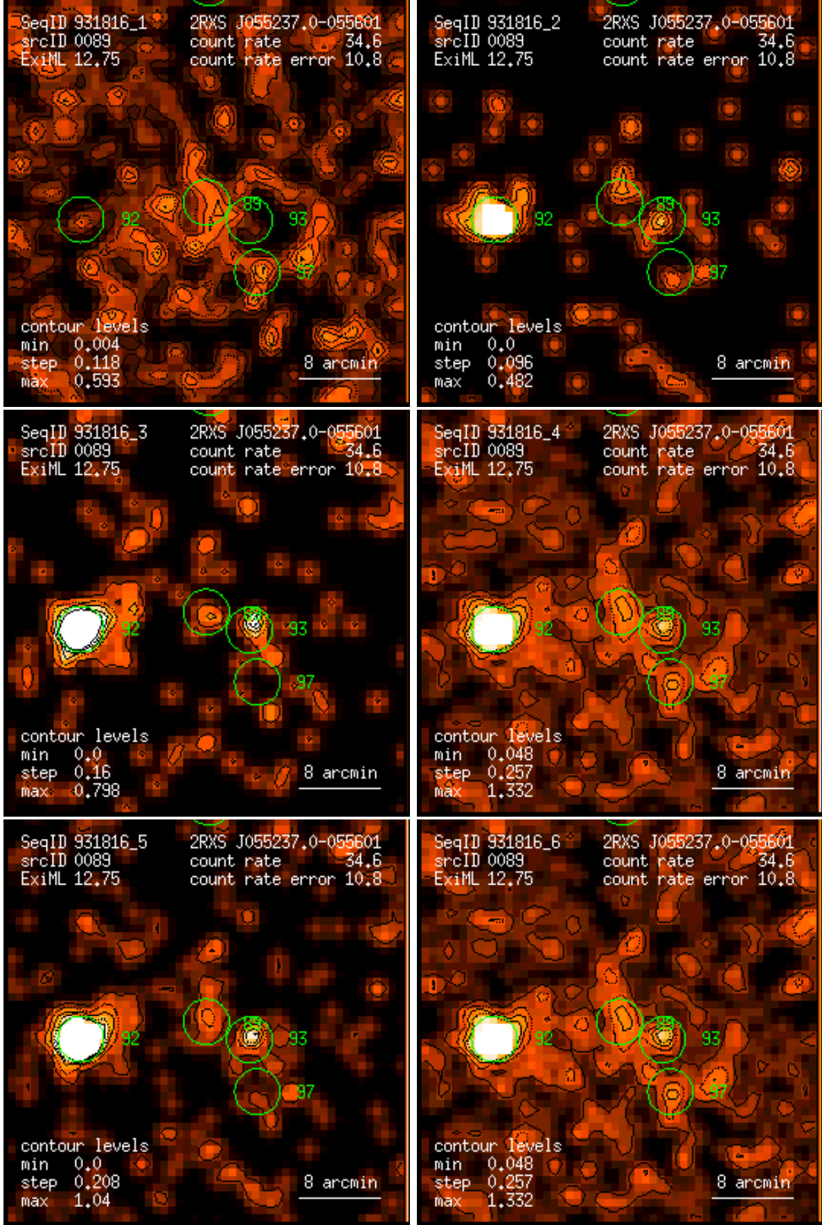
Figure 89: RASS 931816: detection 0089: band rate images, Gaussian filter: (1) PSPC channels 11 – 41, (2) 52 – 90, (3) 91 – 201, (4) 11 – 235, (5) 52 – 201, (6) 11 – 201. Broad band rates in counts/ks. Band rate contour levels in counts/ks/arcmin 2 .
