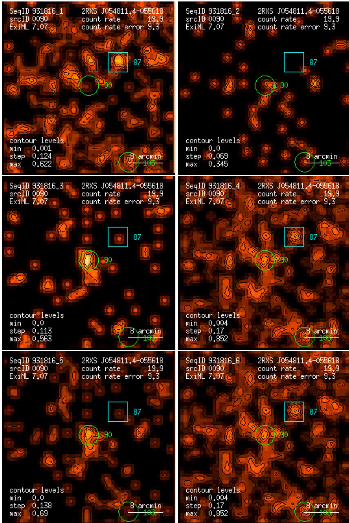
Figure 90: RASS 931816: detection 0090: band rate images, Gaussian filter: (1) PSPC channels 11 – 41, (2) 52 – 90, (3) 91 – 201, (4) 11 – 235, (5) 52 – 201, (6) 11 – 201. Broad band rates in counts/ks. Band rate contour levels in counts/ks/arcmin 2 .
